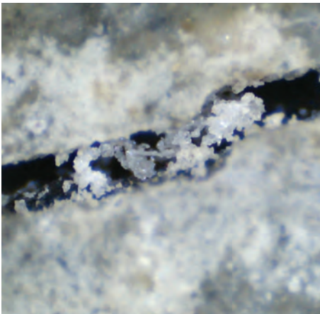
1 week after AQUAFIX application
