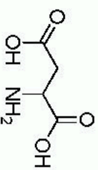
Aspartic Acid
