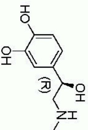
Epinephrine
