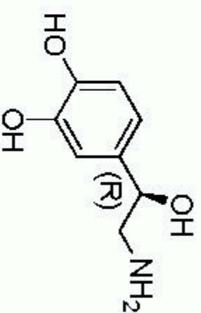
Norepinephrine
