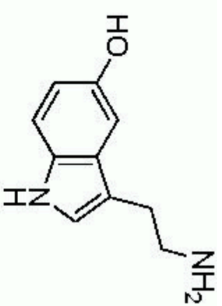
Serotonin
