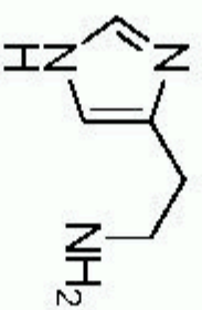
Histamine
