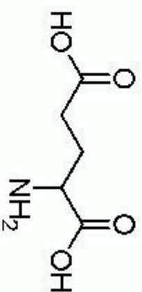
Glutamic Acid
