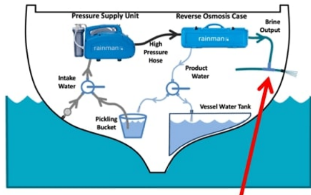
Brine water Tee fitting
