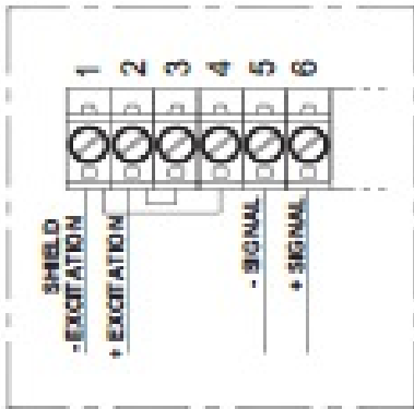
4-wire load cell connection
