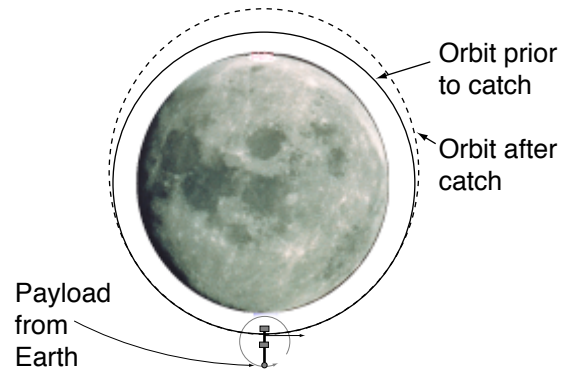
Figure 7. Lunavator™ orbits before and after payload capture.
