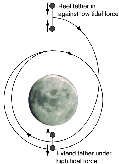
Figure 9. Schematic of tether reeling maneuver to reduce orbital eccentricity.
