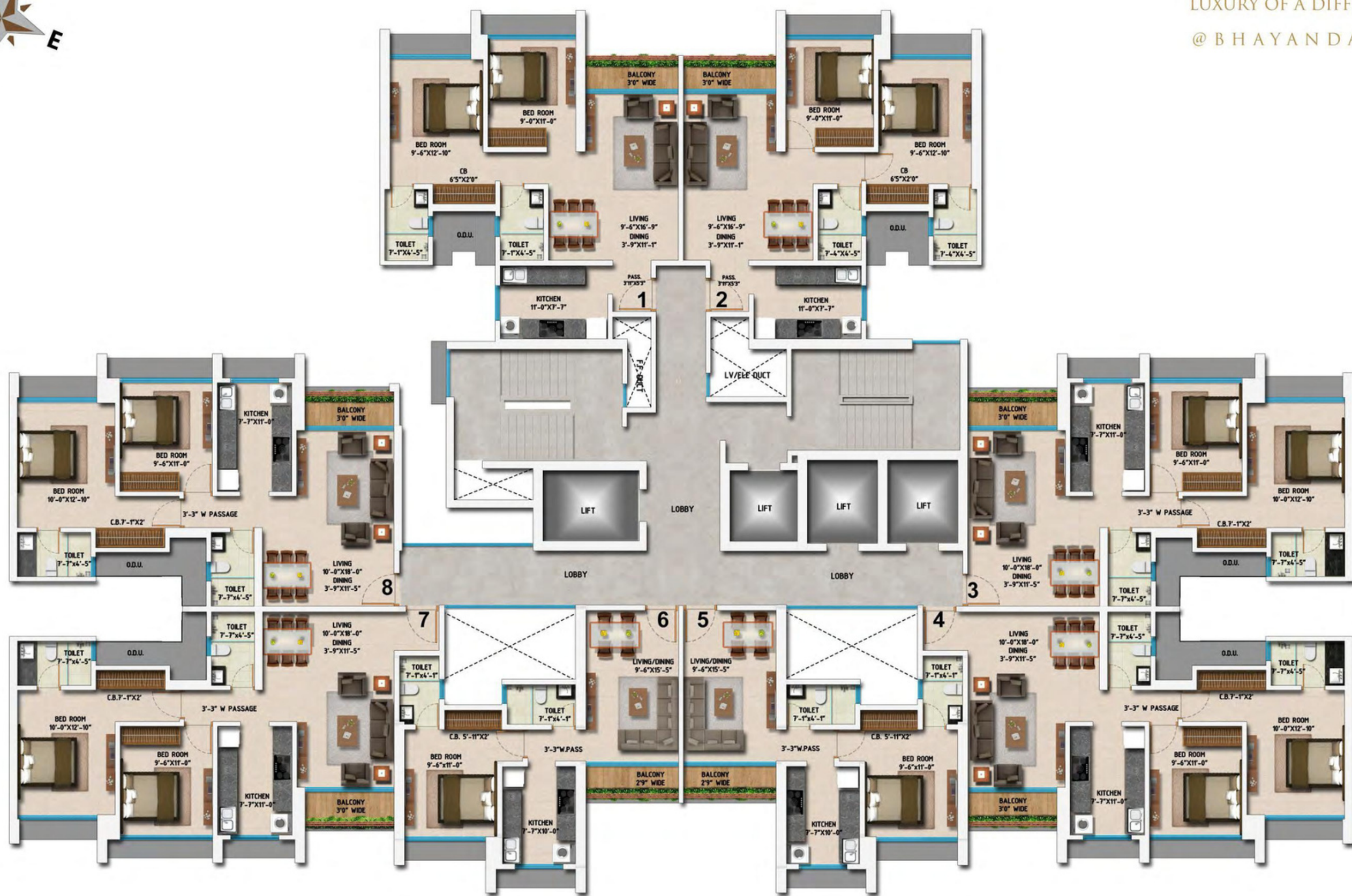
FLOOR PLAN - C WING
