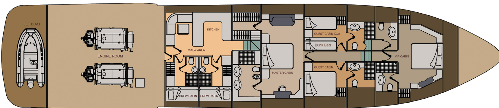
LOWER DECK
