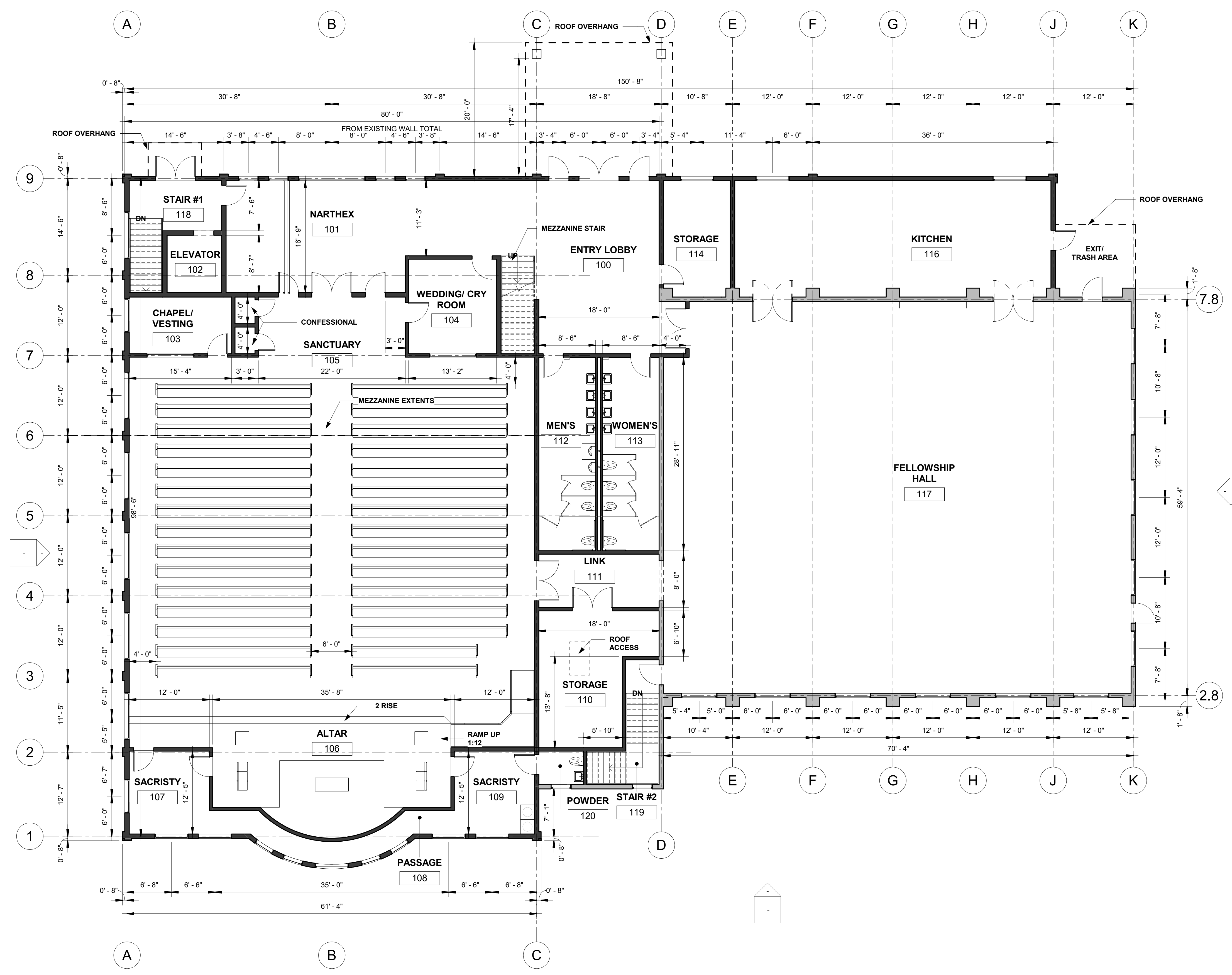
1 MAIN LEVEL 1/8" = 1'-0"
