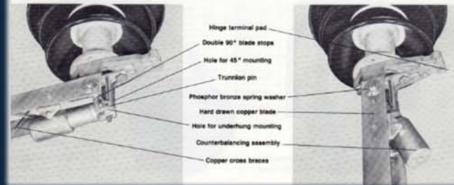
Hinge assembly arrangement of a closed, underhung mounted, switch complete with counterbalancing.
