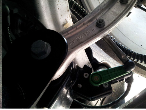
REAR LINKAGE
