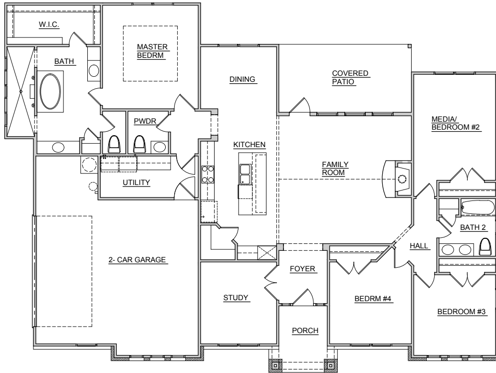
FLOOR PLAN 2358
