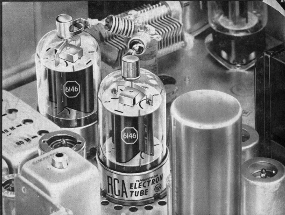
Inside view of the HT-37, showing the two RCA-6146's in parallel in the linear final.
