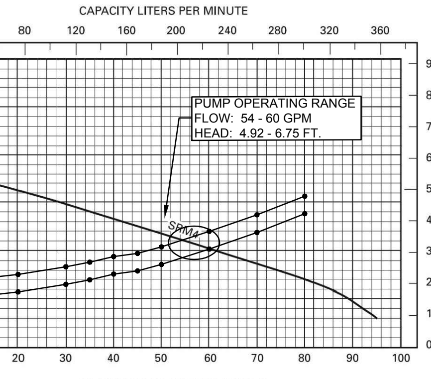
PUMP CURVE: MYERS SRM4
