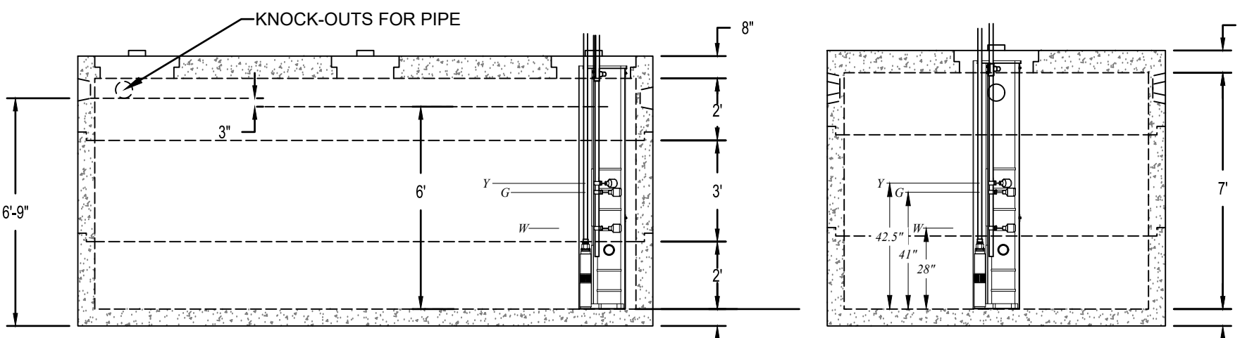
6,000 GALLON RECIRCULATION TANK SCALE 1" = 4'
