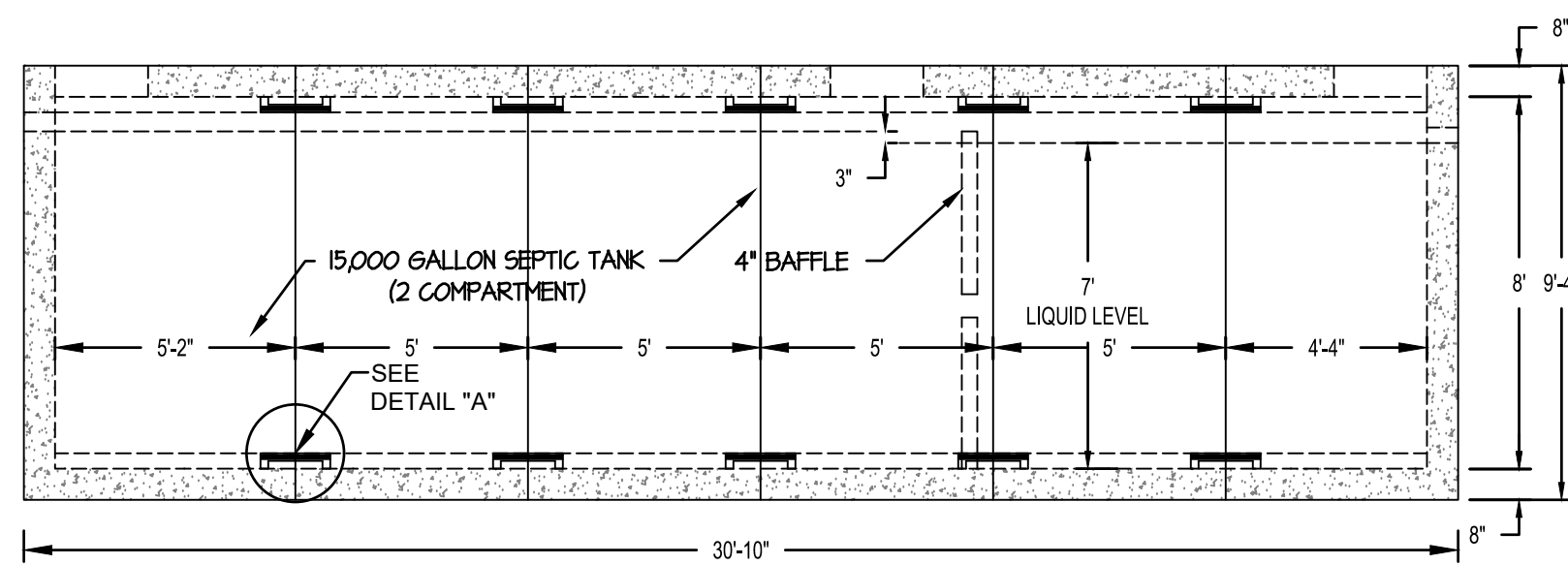
15,000 GALLON TWO COMPARTMENT SEPTIC TANK
