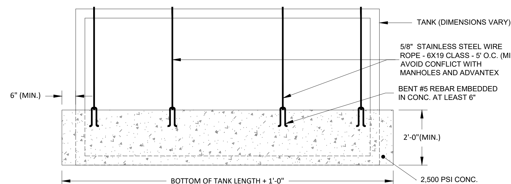
COUNTER WEIGHT: TANK ANTI-FLOATATION SECTIONS
