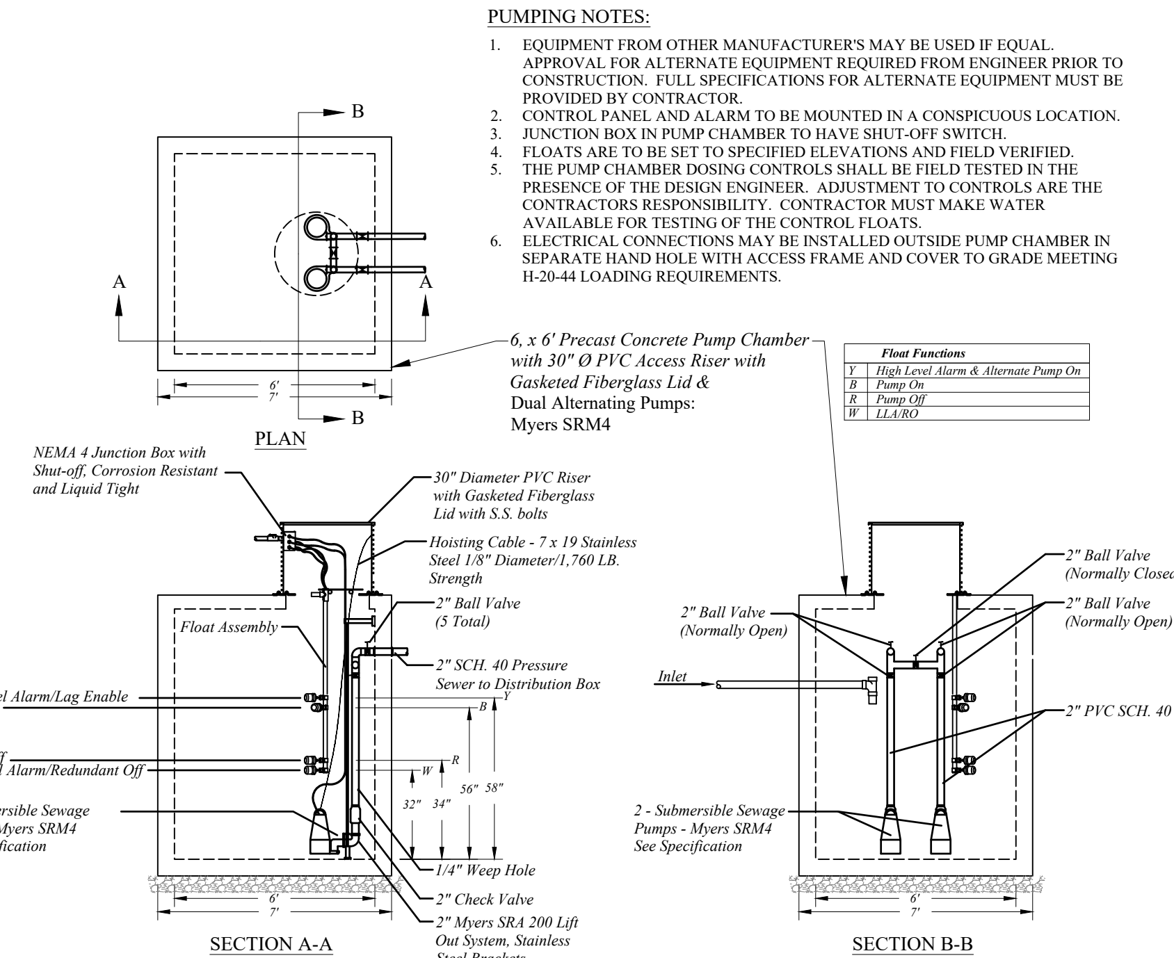
PUMP CHAMBER DETAIL SCALE 1" = 4'
