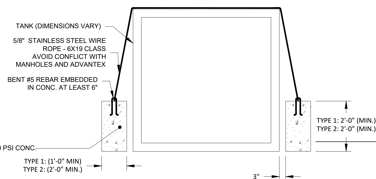
COUNTER WEIGHT: TANK ANTI-FLOATATION SECTIONS
