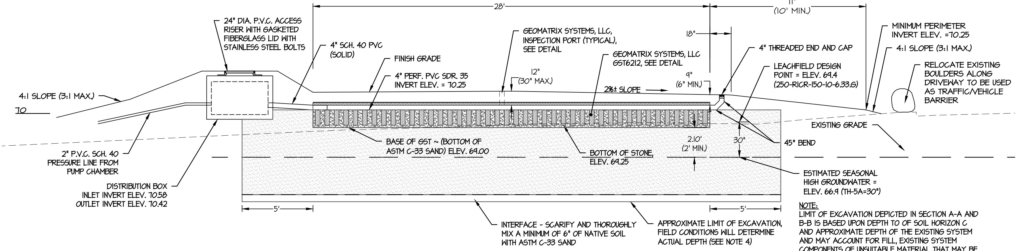
GRAVEL TREATMENT SYSTEM (GST) SECTION A-A SCALE 1" = 4'
