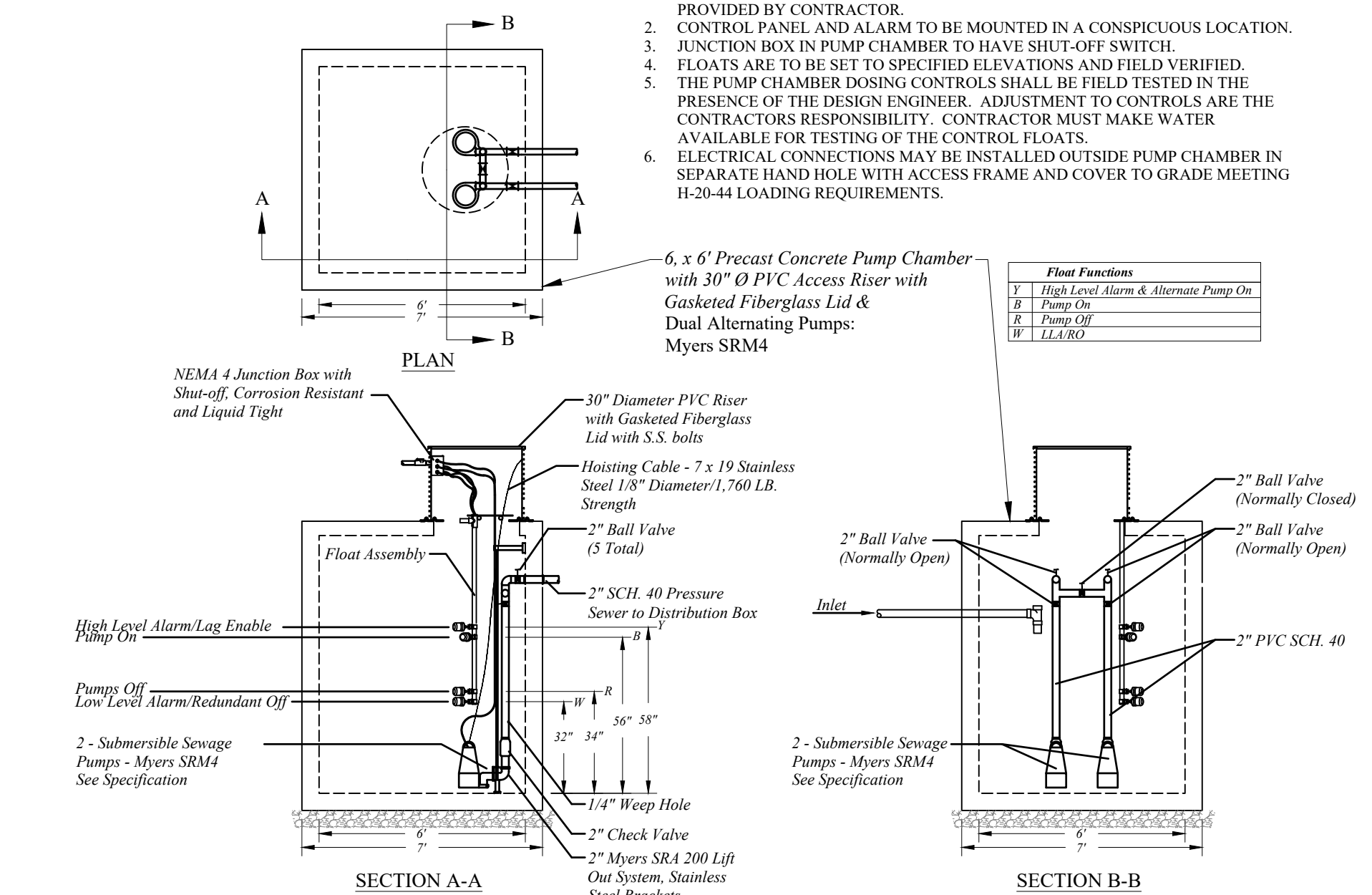
PUMP CHAMBER DETAIL SCALE 1" = 4'
