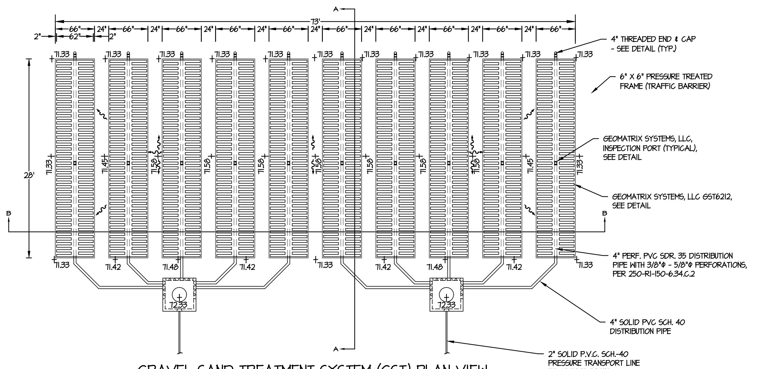
GRAVEL SAND TREATMENT SYSTEM (GST) PLAN VIEW SCALE 1" = 8'
