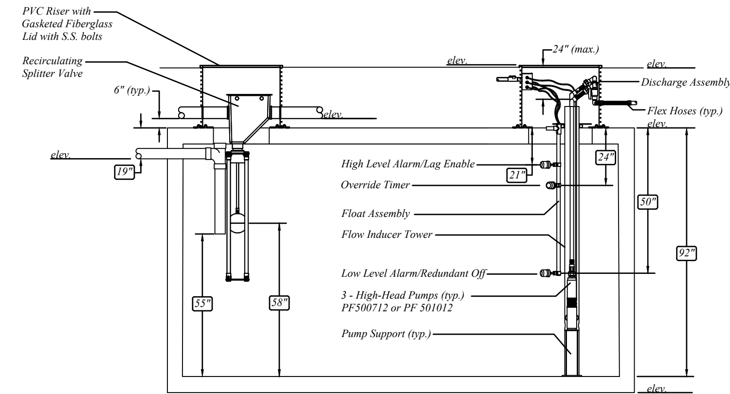
RECIRCULATION TANK FLOAT AND RSV SETTINGS
