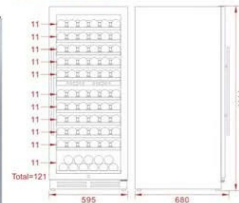
SRW-128D Product(W*D*H)mm
