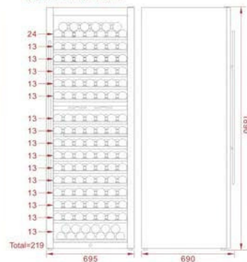
SRW-230D Product(W*D*H)mm
