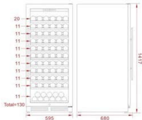
SRW-128S Product(W*D*H)mm
