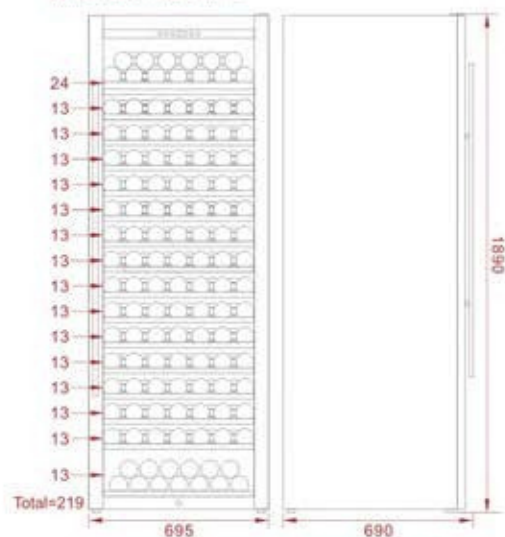
SRW-230S Product(W*D*H)mm
