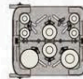
Layout for 7" by 9" trays 4.5" and 5.5" to 7" plates
