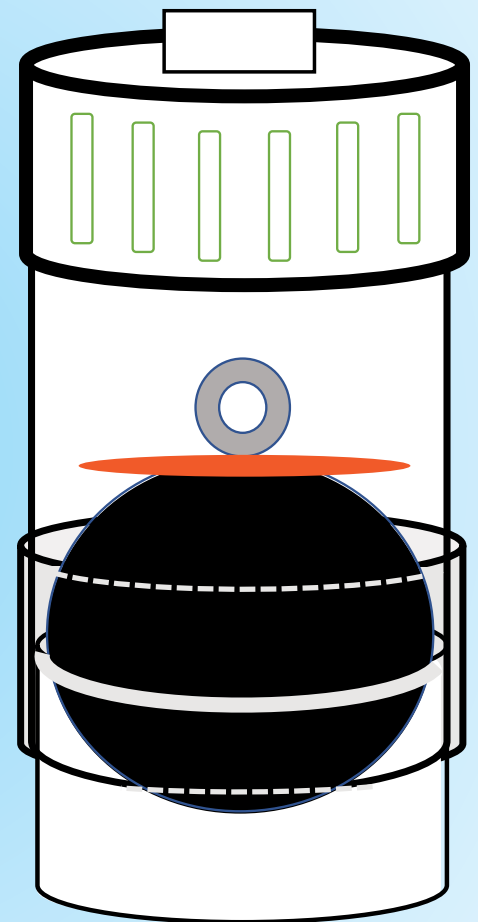
Plug shown with Locator (Smart Plug). Cross Section View. (Drawing Not To Scale)
