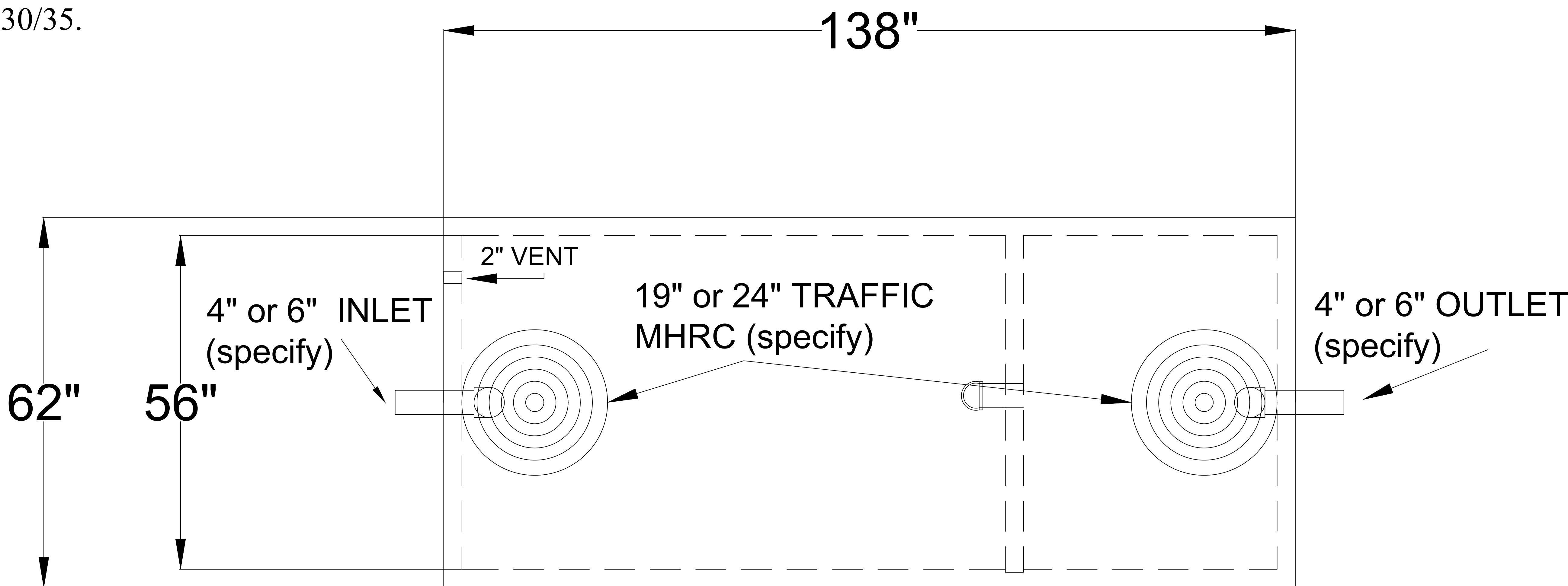
TOP VIEW
