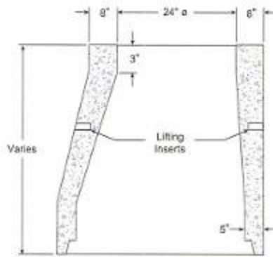
Eccentric Cone 24" \phi Opening
