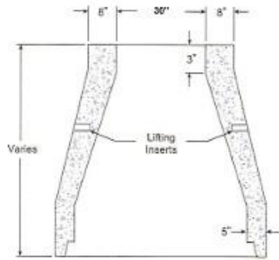
Concentric Cone 30" Opening
