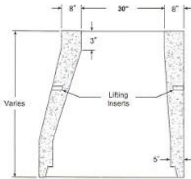
Eccentric Cone 30" Opening
