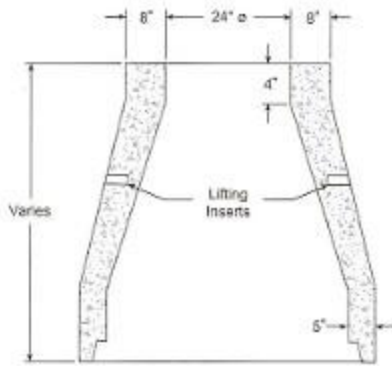
Concentric Cone 24" \phi Opening
