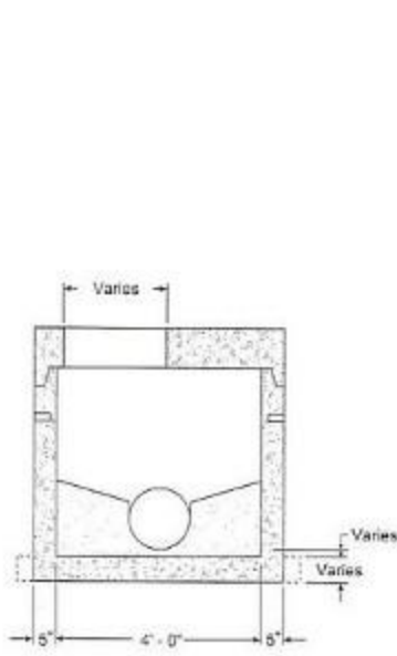
Flattop Illustration for Shallow Manhole
