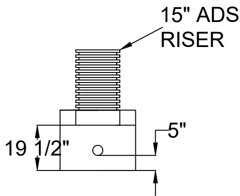
INLET/OUTLET VIEW
