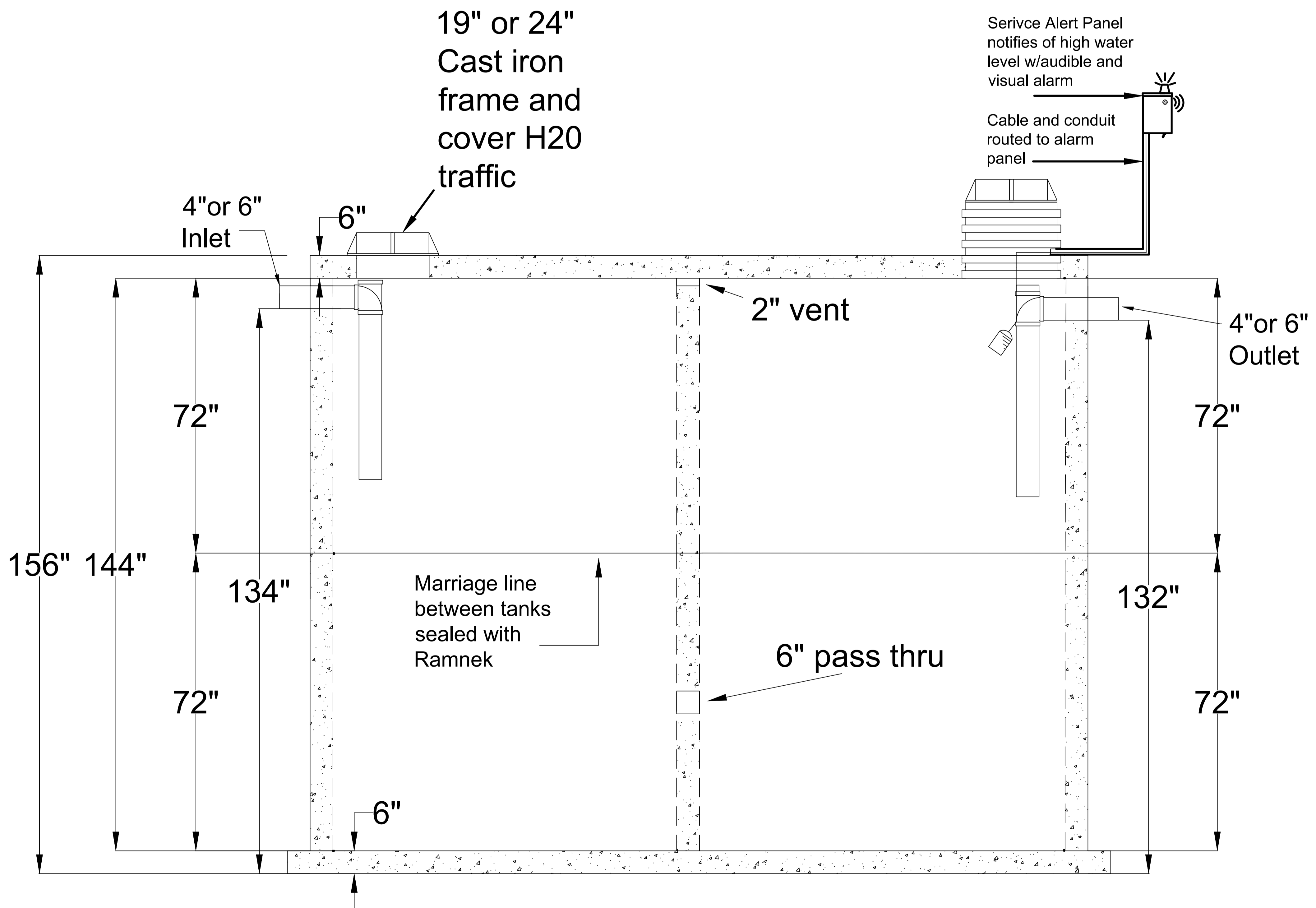
SIDE VIEW
