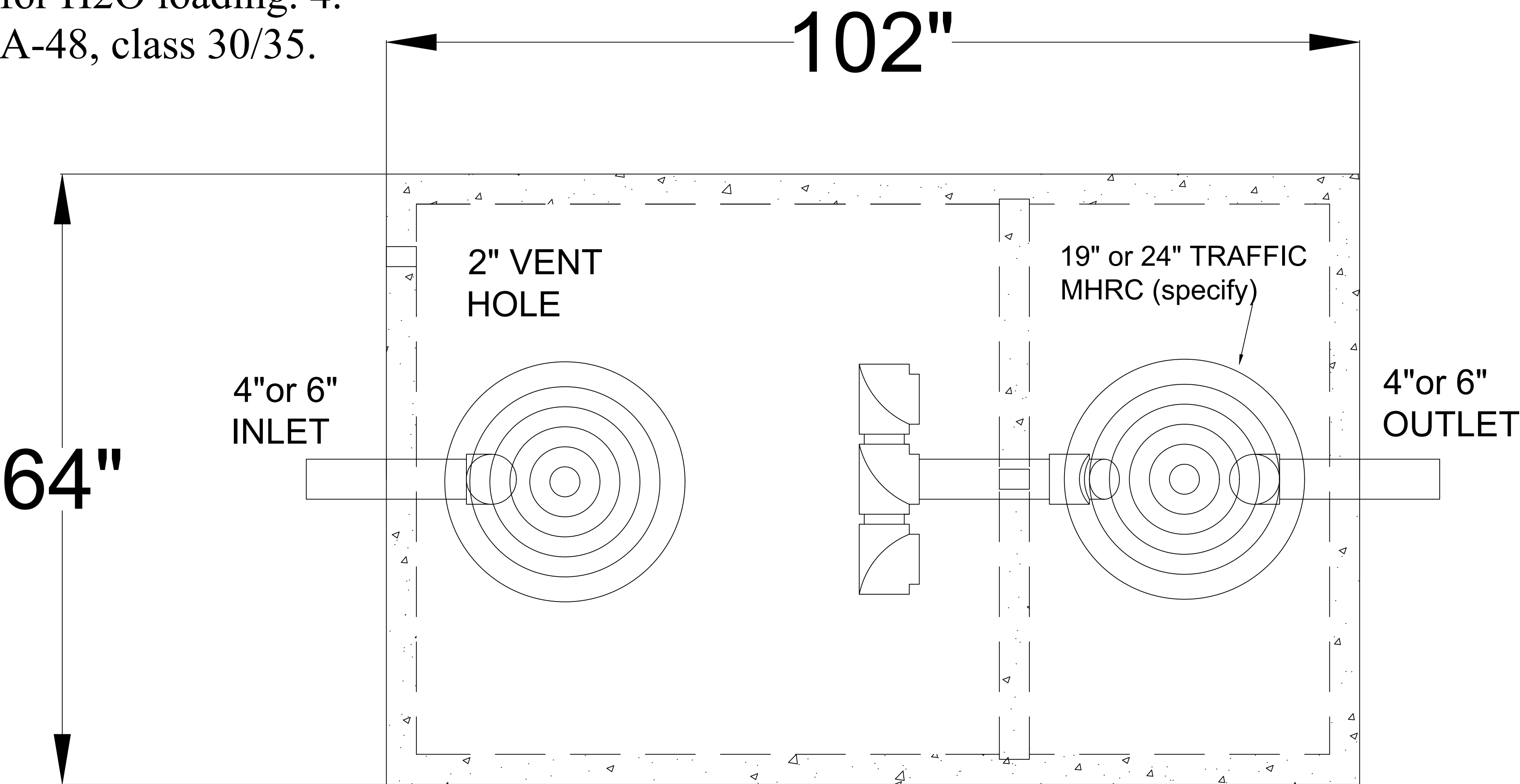
TOP VIEW
