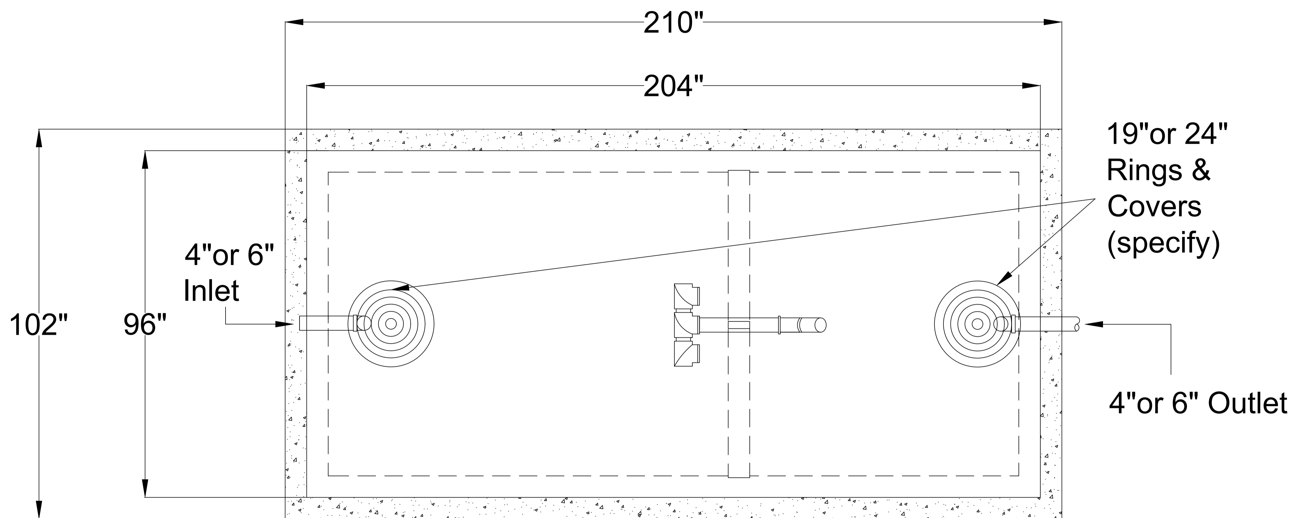
TOP VIEW
