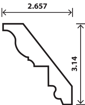
CR 11 3/4" x 4 1/8"
