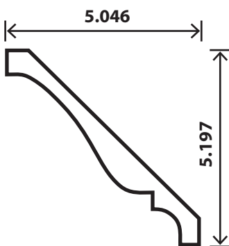
CR 72 13/16" x 7 1/4"
