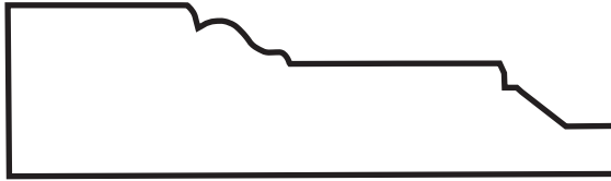
Base 49 3/4" x 3 1/4"
