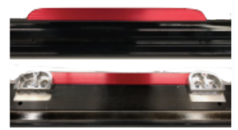
Air Ride End Rail with RED Goal Bar and Spacers- Welded with Rubber Trim Part Number: 3207561W-REDBAR
