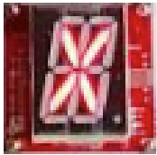
QuadAir V4 Life Digital Display Board (Under Playfield) NEW Part Number: 3612423
