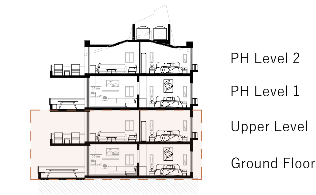
Building Section
