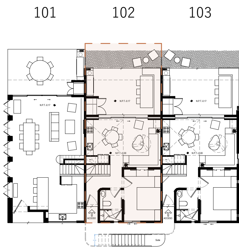
Building Ground Floor Plan
