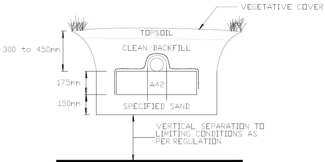
Figure 4: Vertical Separation to Limiting Conditions
