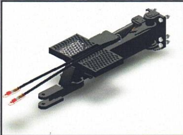
Removable Bolted Cylinder Drawbar
