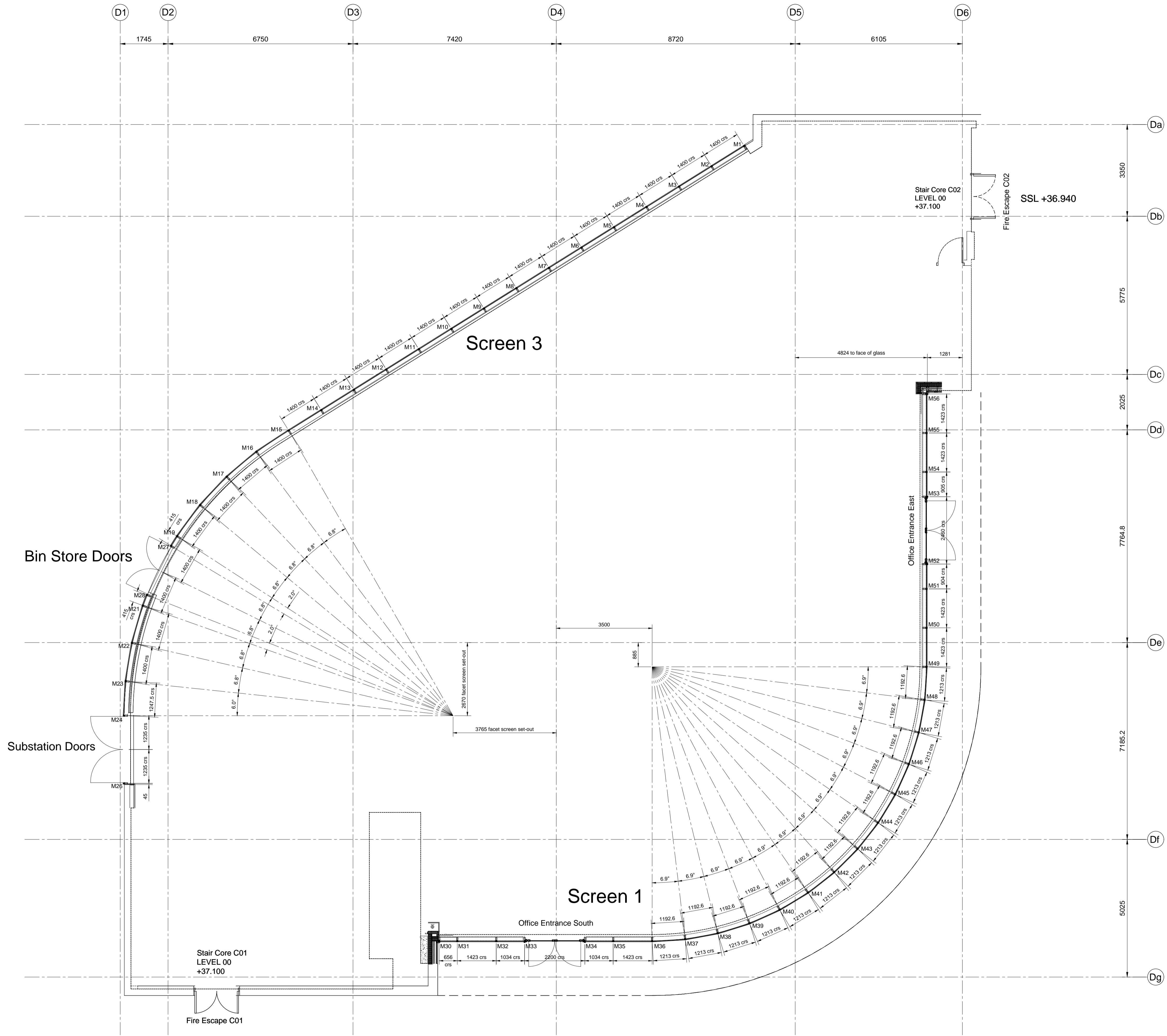
Plan Set-Out Through Curtain Wall Screens 1 & 3 At Ground to Underside Of 2nd Floor
