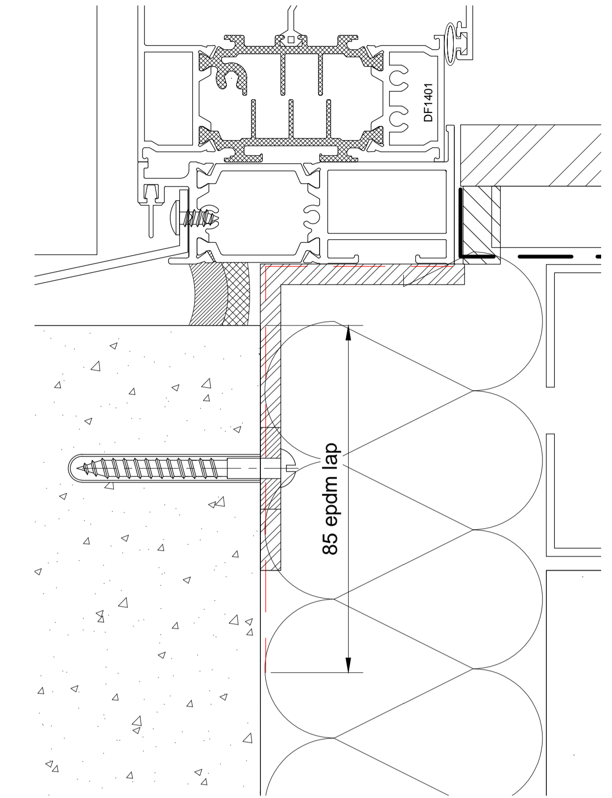
EPDM Coverage Details
