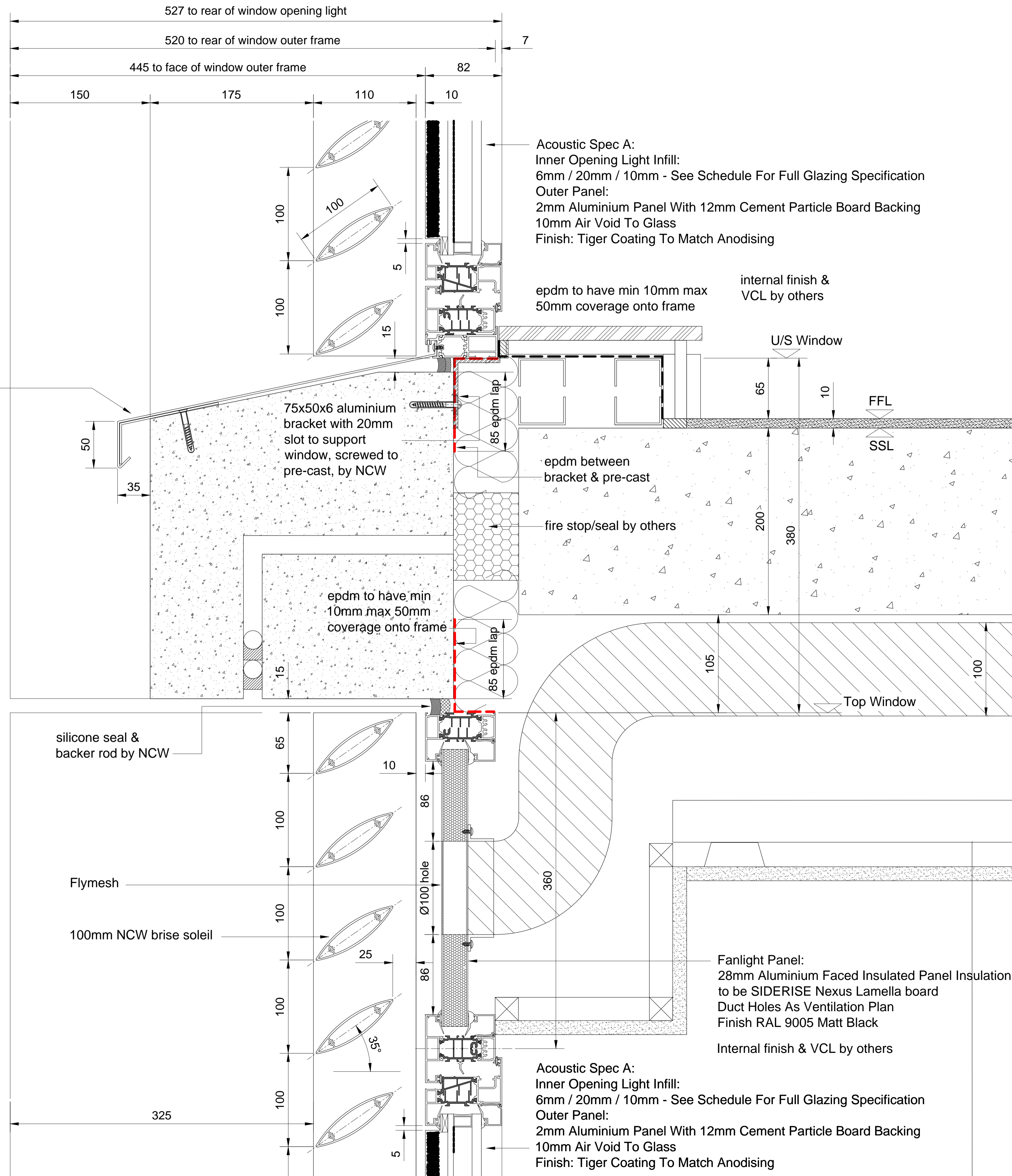
2 D01 Brise Soleil Frame Head Detail
