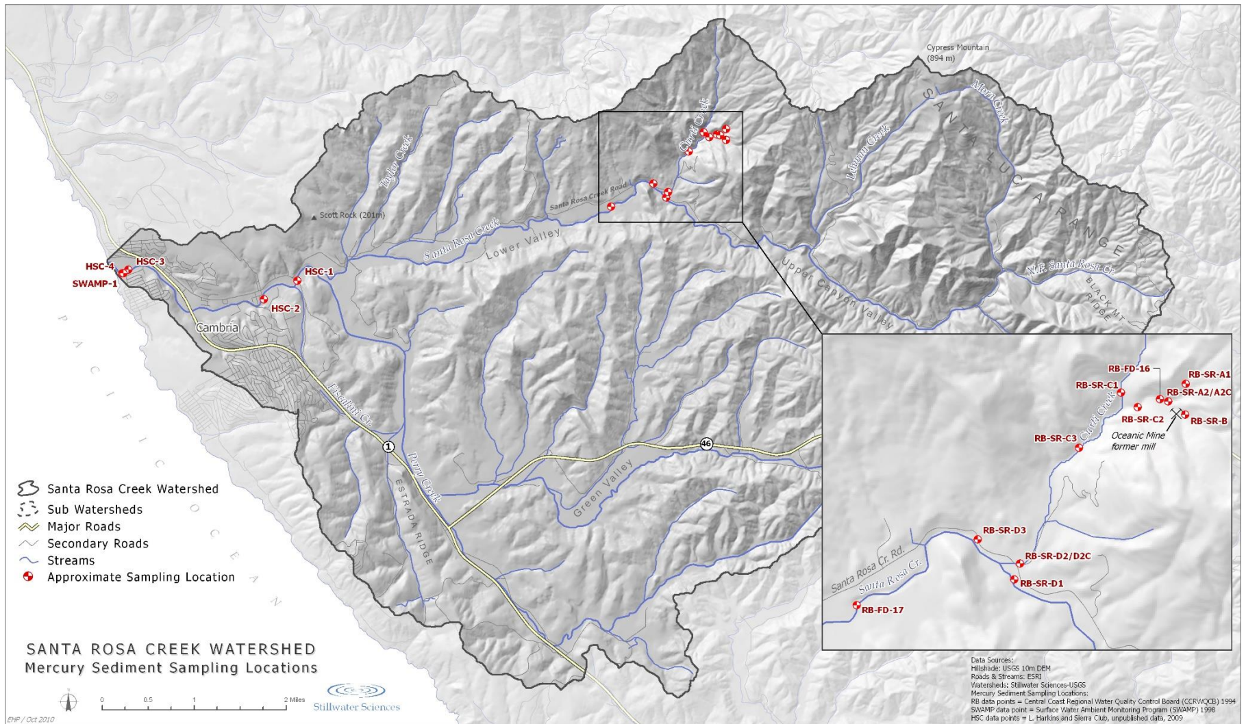
Figure 2.13 Mercury Sampling
