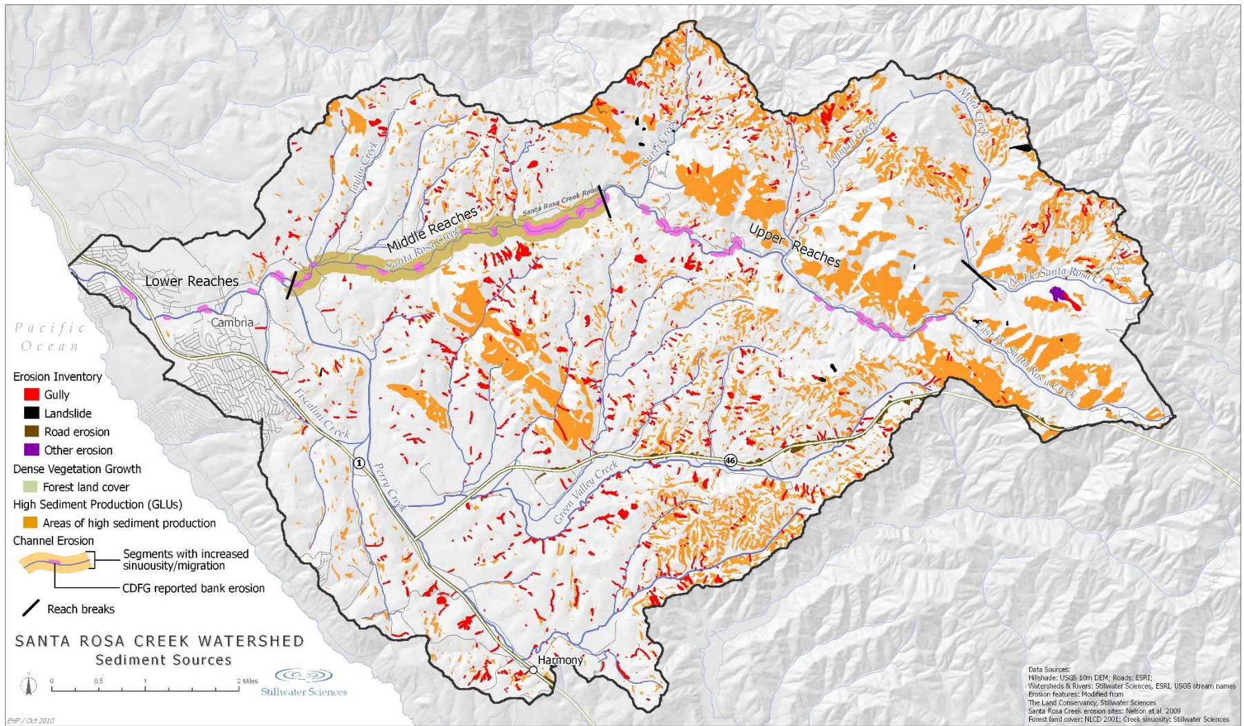
Figure 2.8 Sediment Sources
