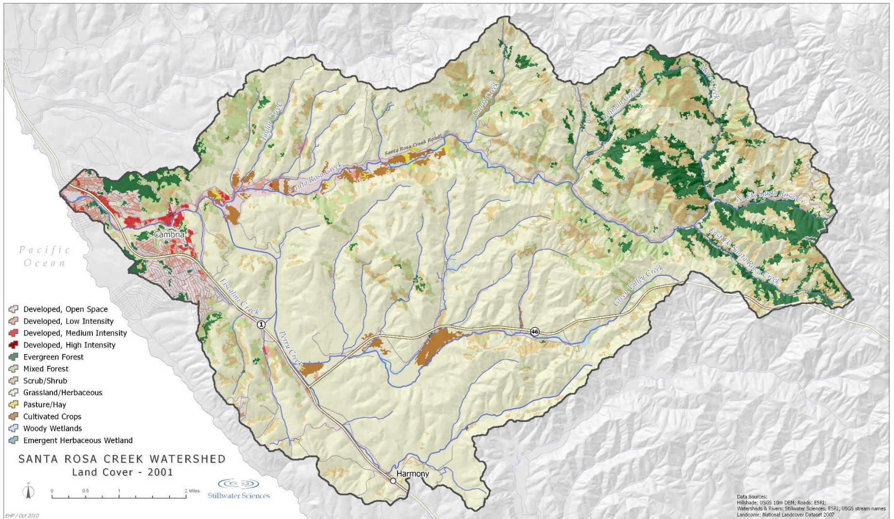
Figure 2.24 Land Cover
