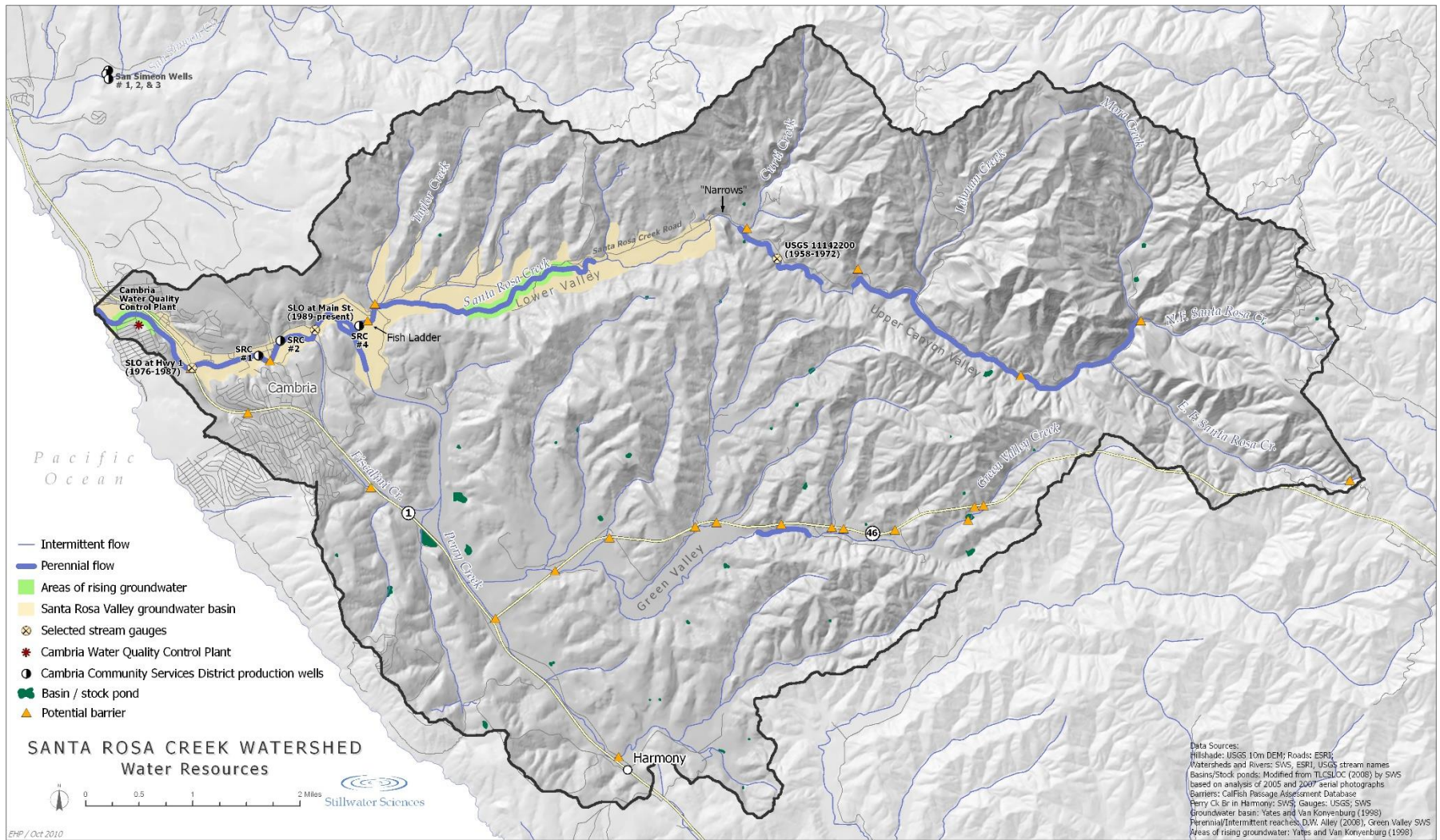
Figure 2.9 Water Resources
