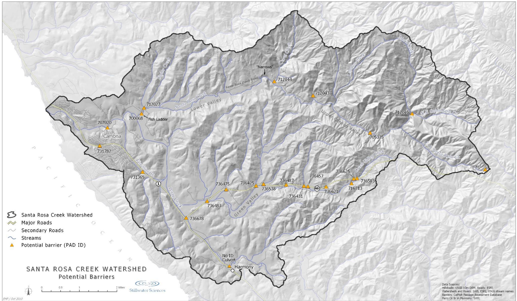
Figure 2.12 Barriers
