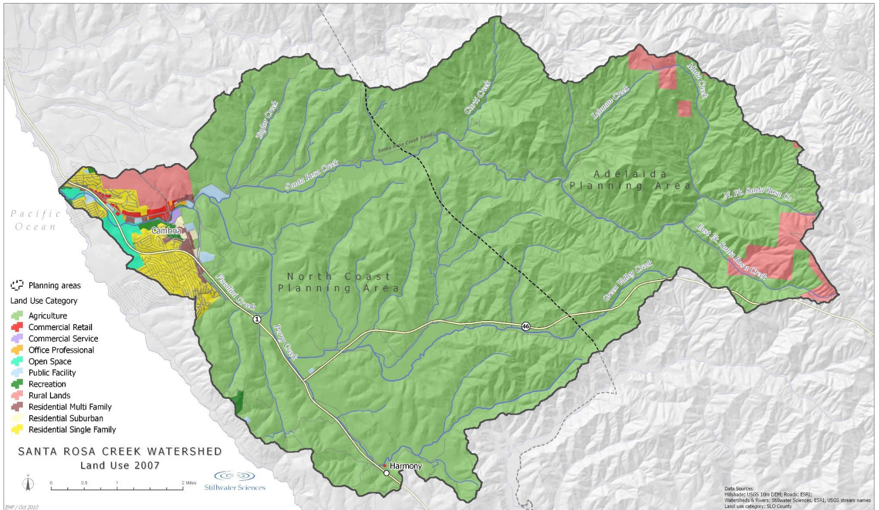
Figure 2.3 Land Use
