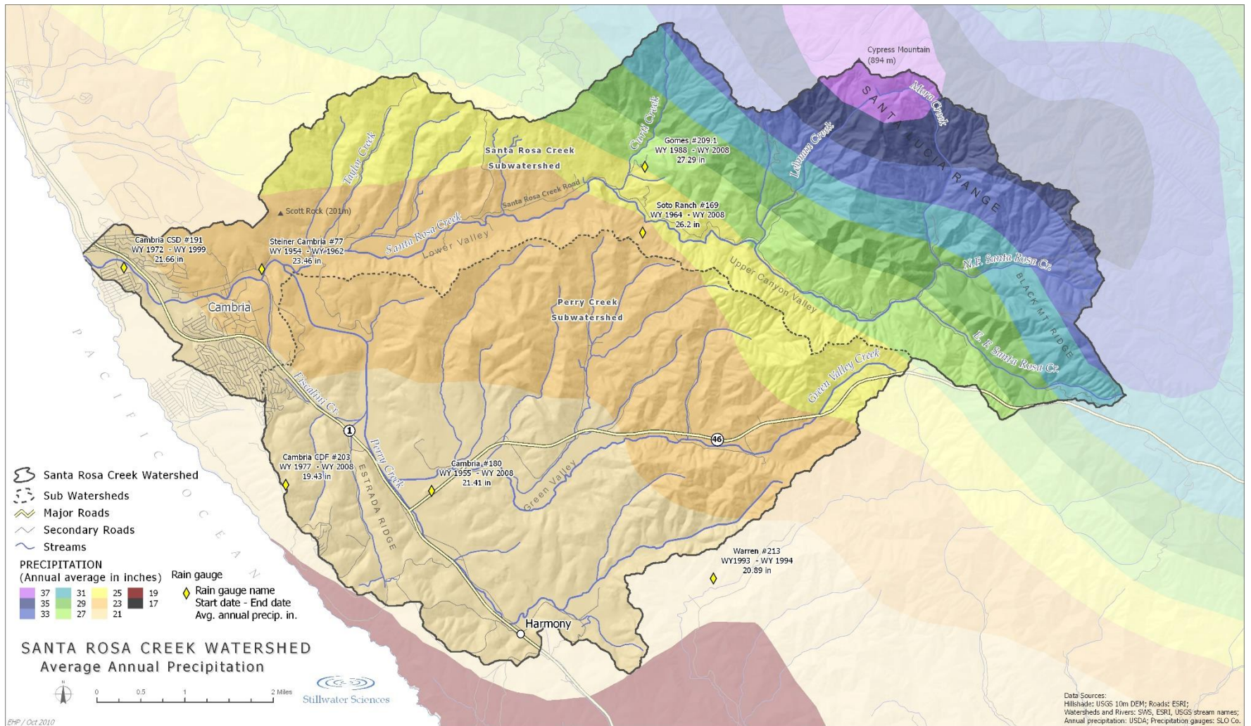
Figure 2.5 Precipitation
