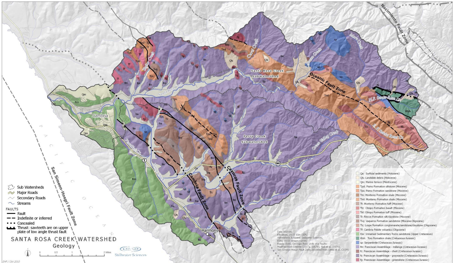
Figure 2.7 Geology
