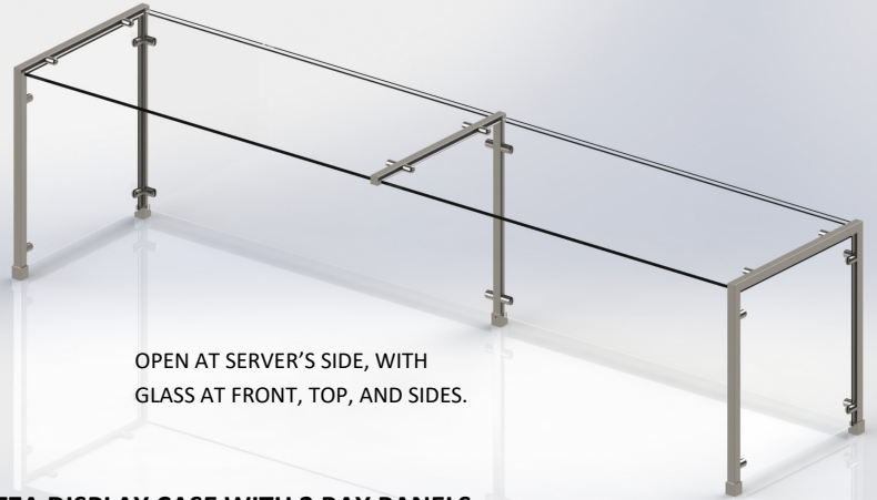
PIZZA DISPLAY CASE WITH 2 BAY PANELS
