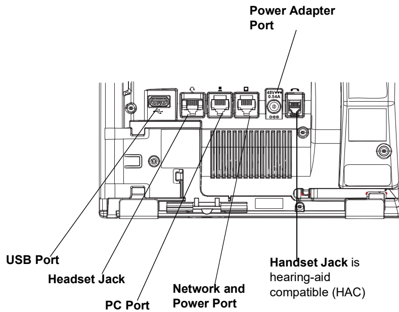
Figure 2: Ports on the Back of the 6930 IP Phone
