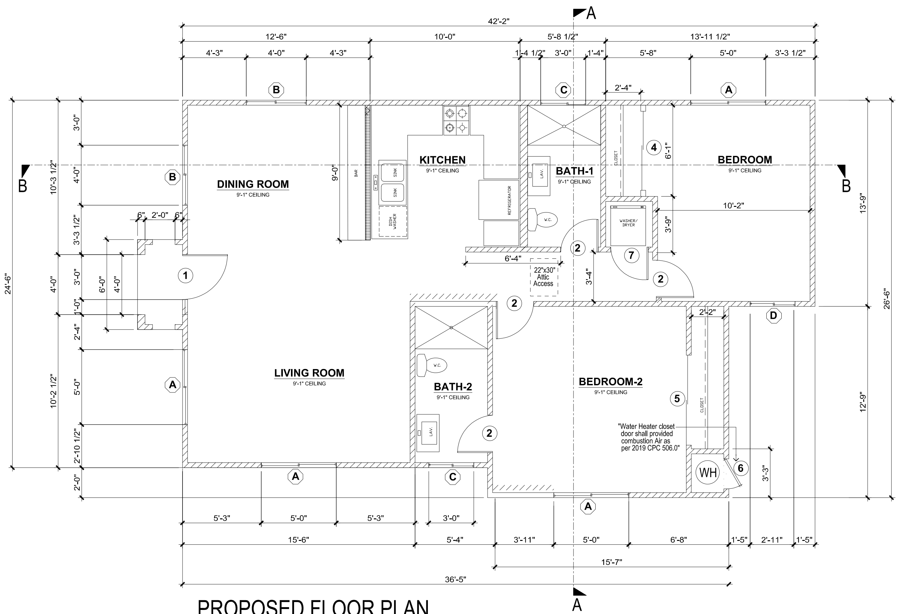
PROPOSED FLOOR PLAN ACCESSORY DWELLING UNIT
