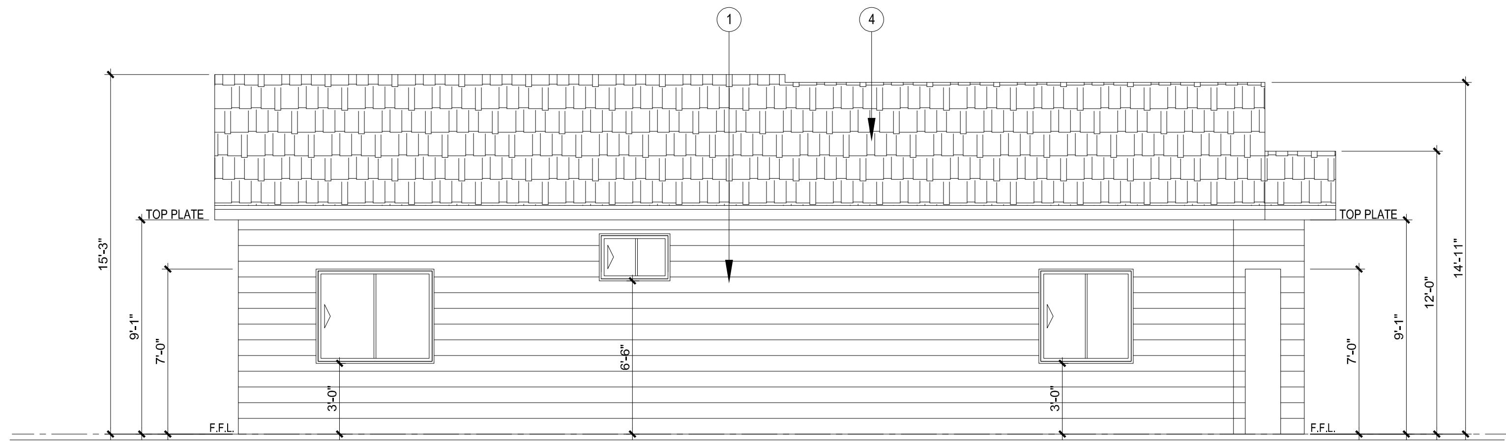
PROPOSED LEFT SIDE ELEVATION ACCESSORY DWELLING UNIT SCALE : 1/4" = 1'-0"
