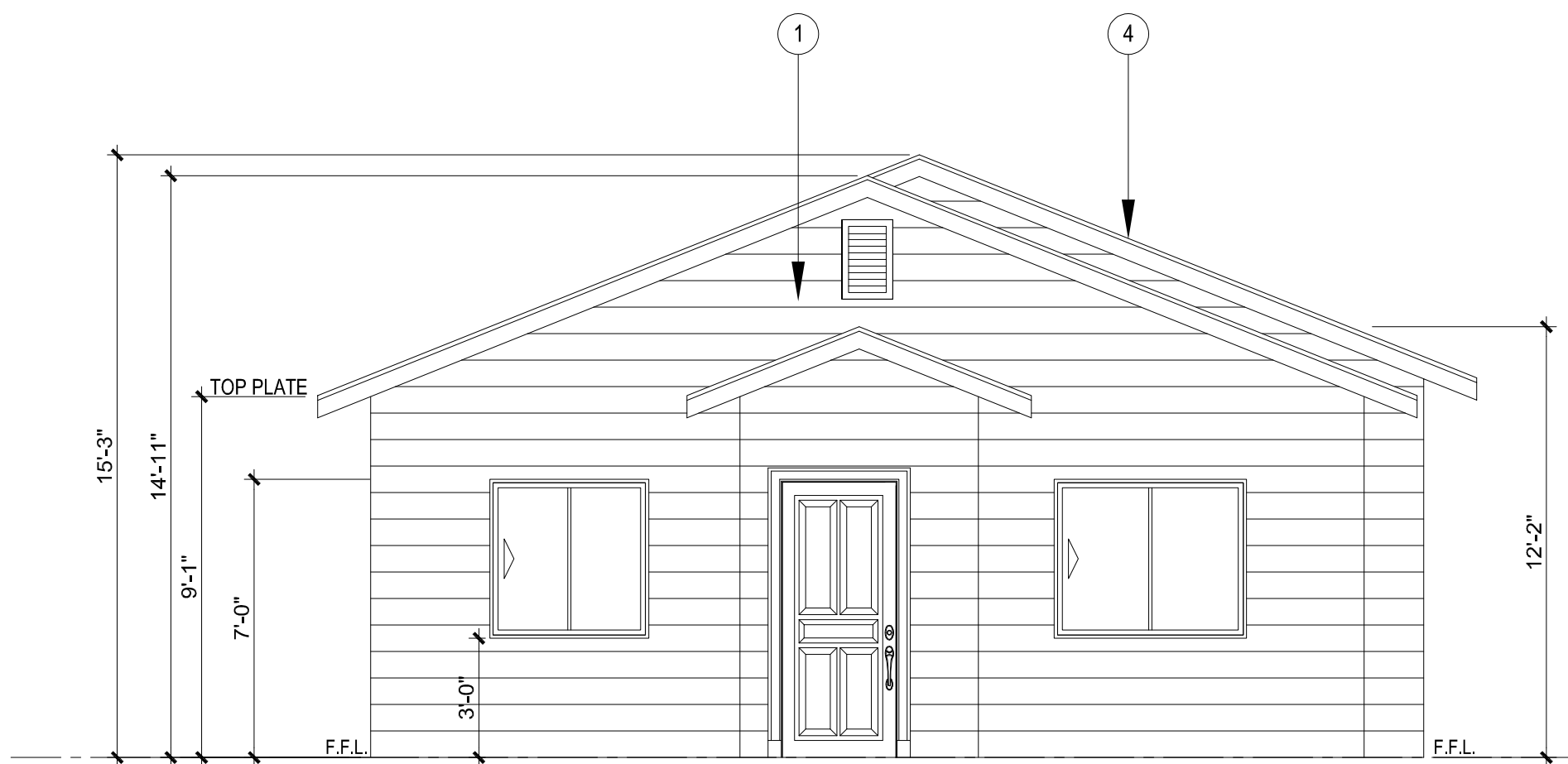
PROPOSED FRONT ELEVATION ACCESSORY DWELLING UNIT SCALE : 1/4" = 1'-0"
