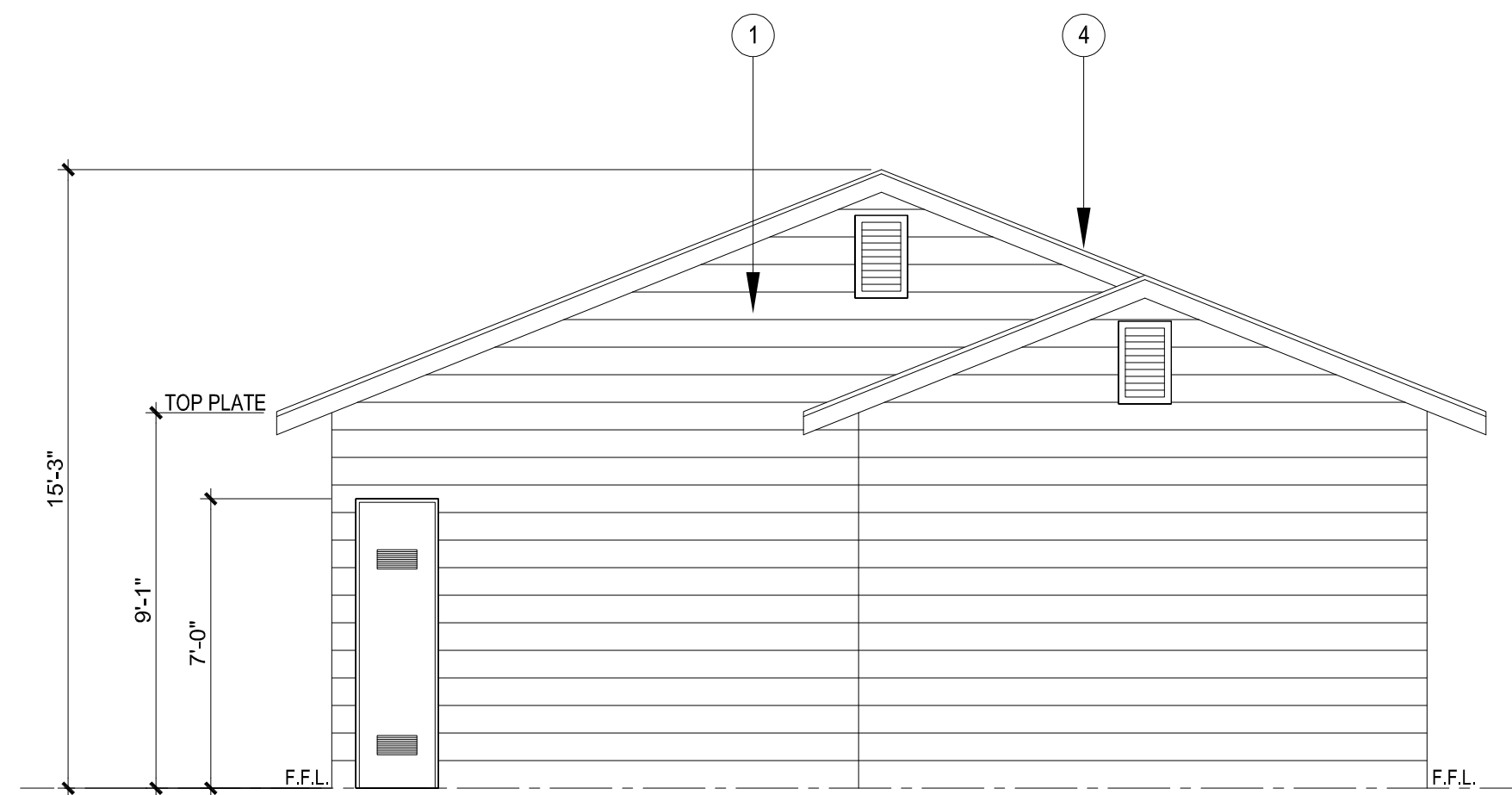
PROPOSED REAR ELEVATION ACCESSORY DWELLING UNIT SCALE : 1/4" = 1'-0"
