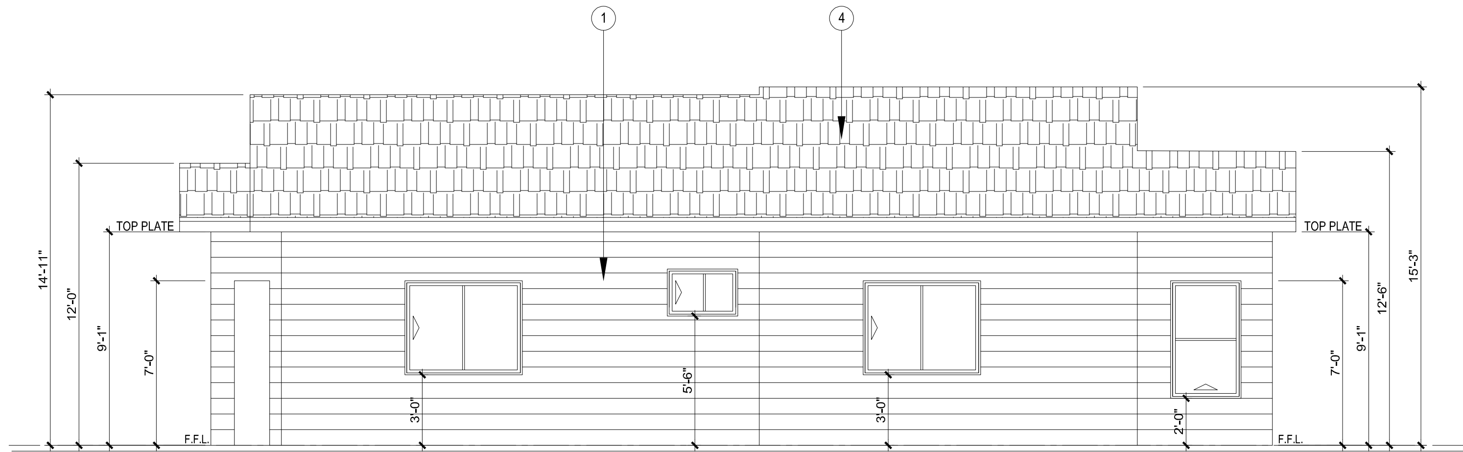
PROPOSED RIGHT SIDE ELEVATION ACCESSORY DWELLING UNIT SCALE : 1/4" = 1'-0"
