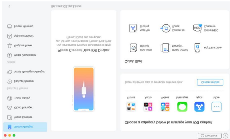
AnyTrans Overview
