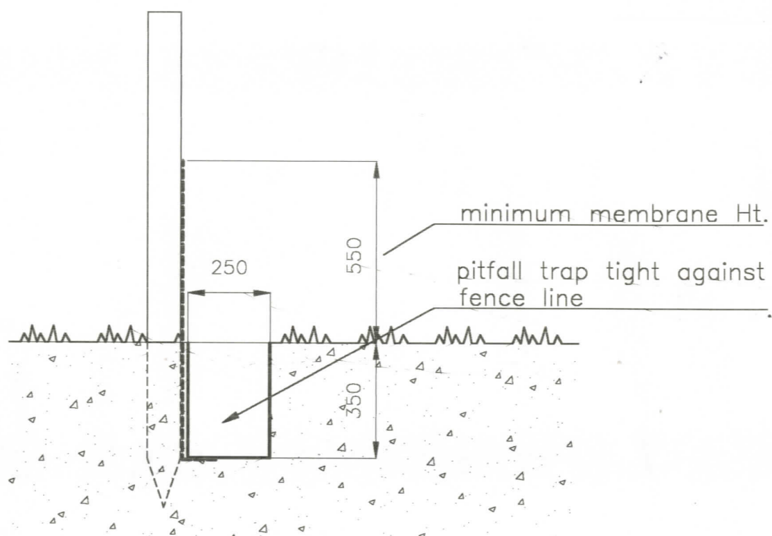
section
