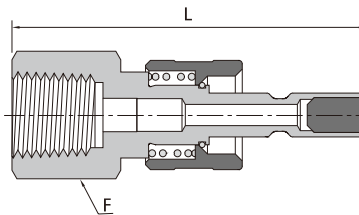
NPT 阴螺纹
