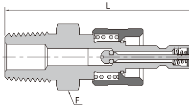
BSPT阳螺纹
