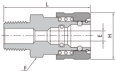
NPT 阳螺纹
