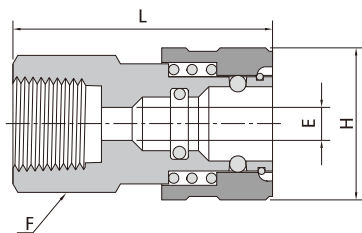
NPT 阴螺纹
