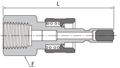
BSPT 阴螺纹
