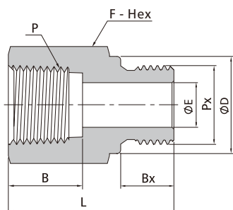
Female NPT Threads
