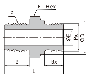
Male NPT Threads
