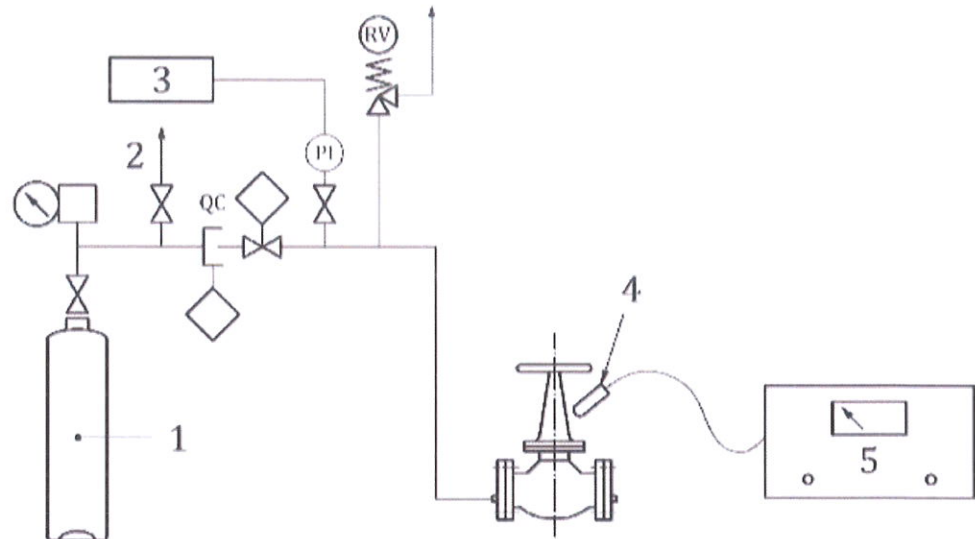
Figure 2 Typical body seal leakage measurement system with Sniffing Method
