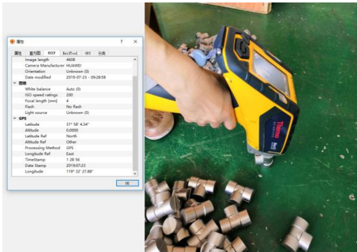
Niton Portable spectrometer
