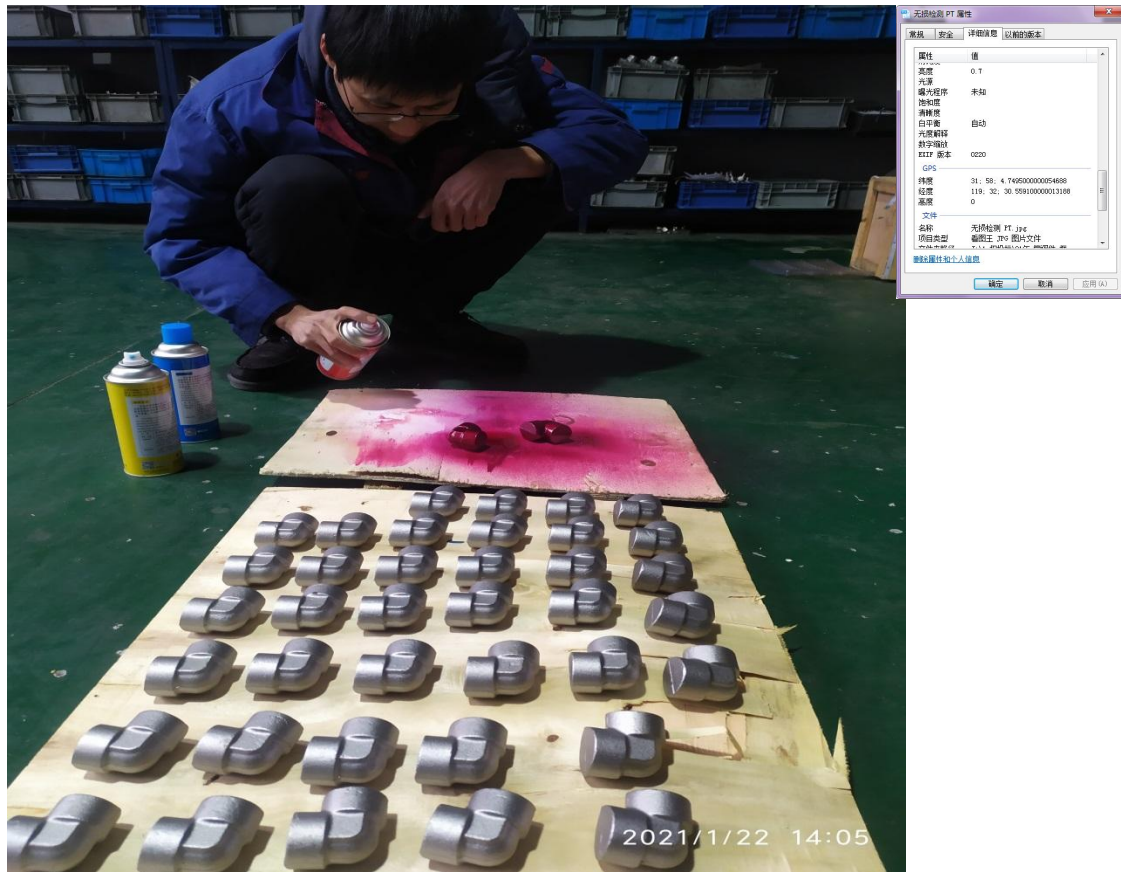
Nondestructive examination PT
