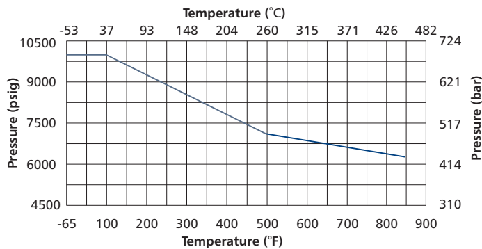
Valve Body with 316 SS
