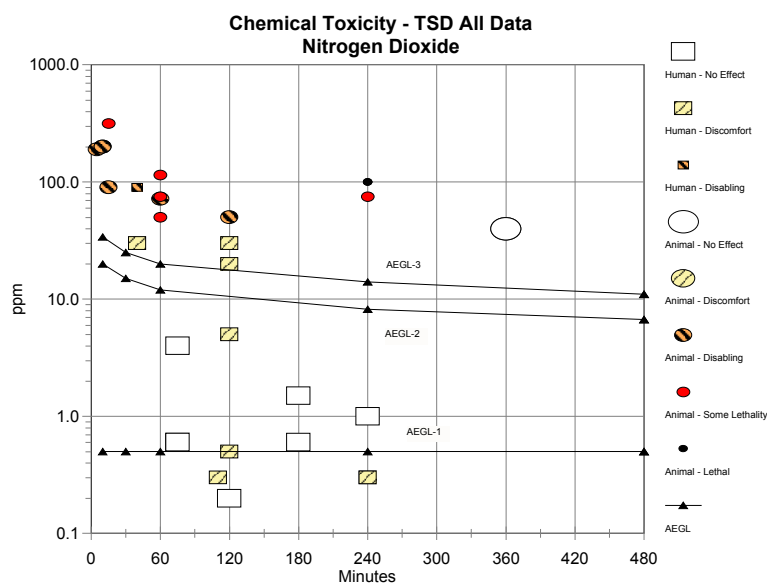
FIGURE C-1 Category plot of toxicity data and AEGLs values for nitrogen dioxide.
