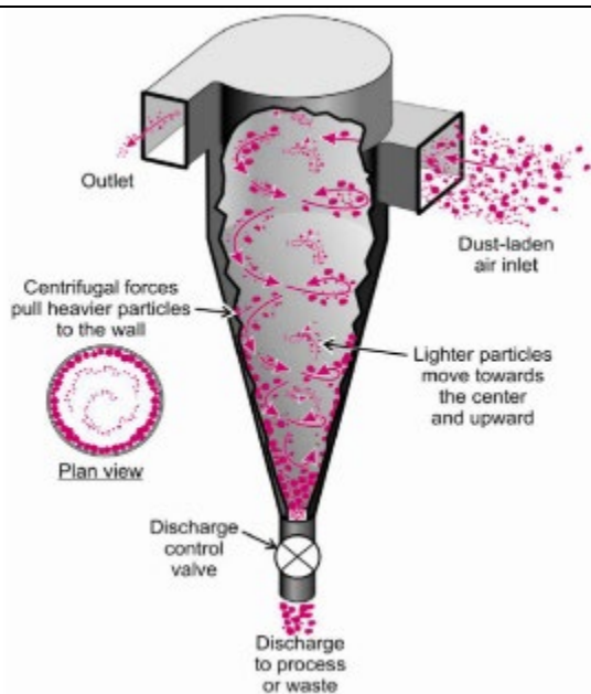
Cyclone Operation (Source: https://www.researchgate.net/figure/Typical-design-of-a-cyclone-dust-collector_fig12_318967816 )
