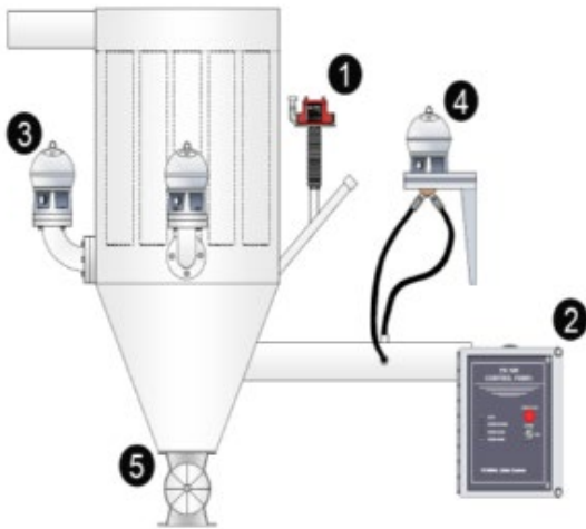
Chemical Suppression System (Source: Fenwal)
