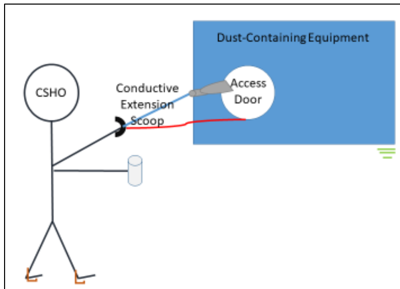
Figure VIII-8: Sampling low-MIE dusts from inside equipment. LOTO by employer with no confined space entry required. This should be a rare occurrence. (Source: OSHA HRT)
