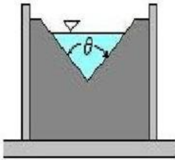
Figure 40. Cross sectional view of v-notch weir.
