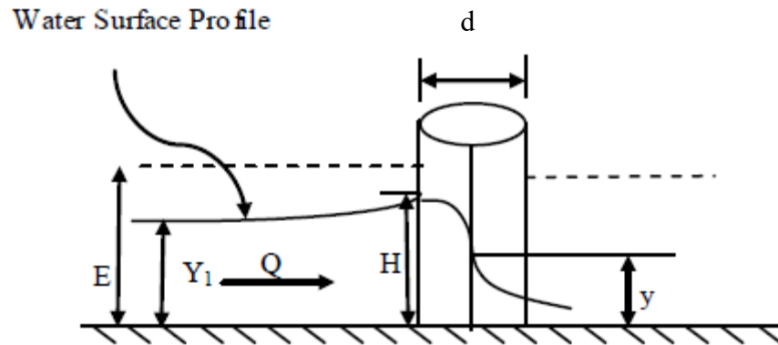
Figure 10. Profile view of S-M rectangular flume (Badar, 2012).
