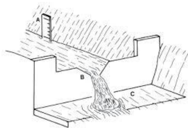
Figure 43. Combination V-notch and contracted rectangular weir.
