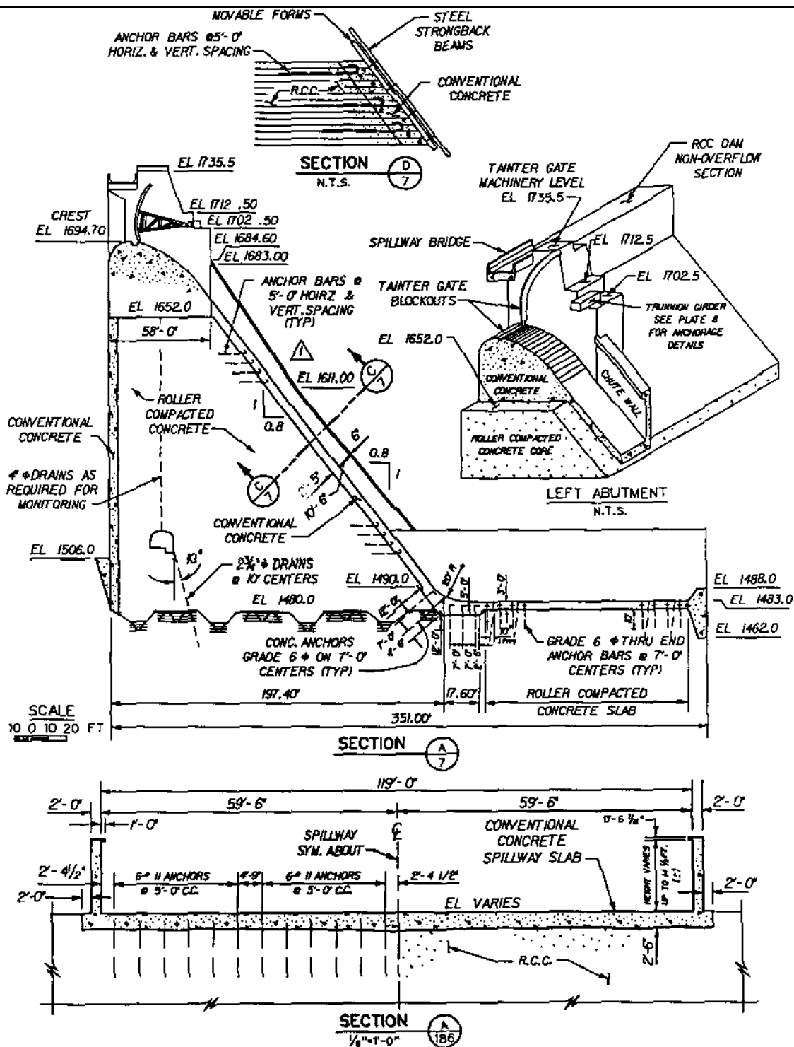
Figure 9-6. RCC spillway details
