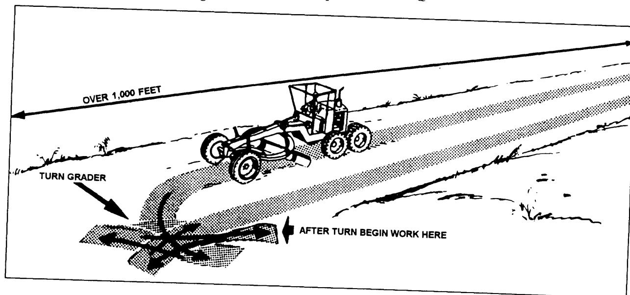
Figure 10-19.-Turning around.
