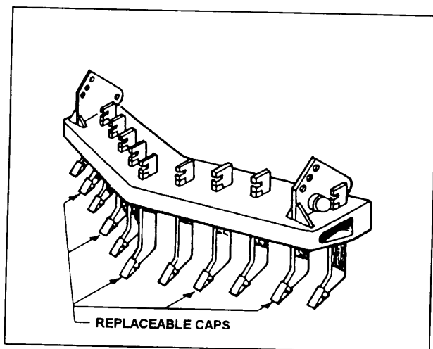
Figure 10-13.-Scarifier teeth.
