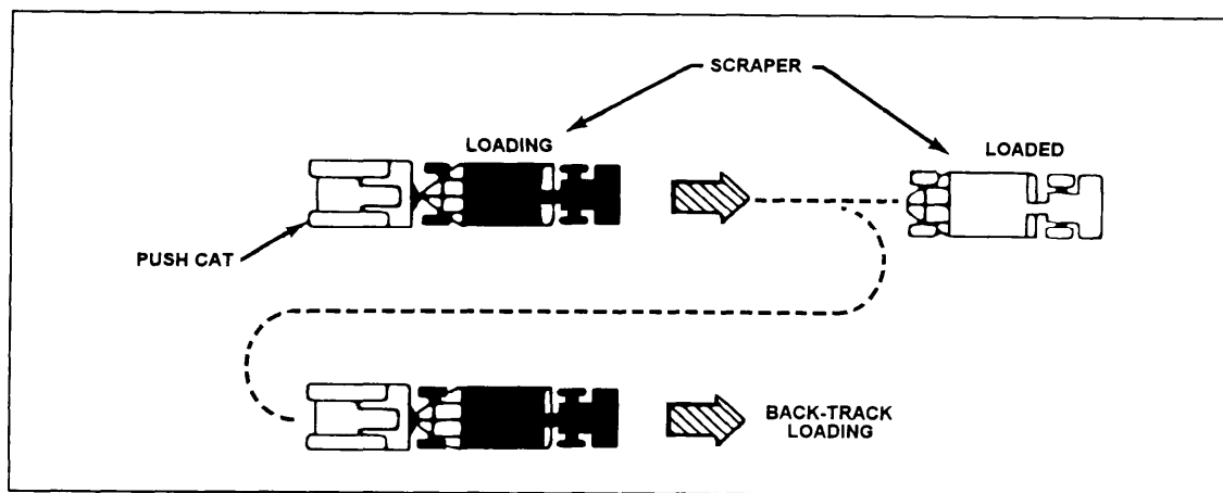
Figure 10-45. Back-track loading.
