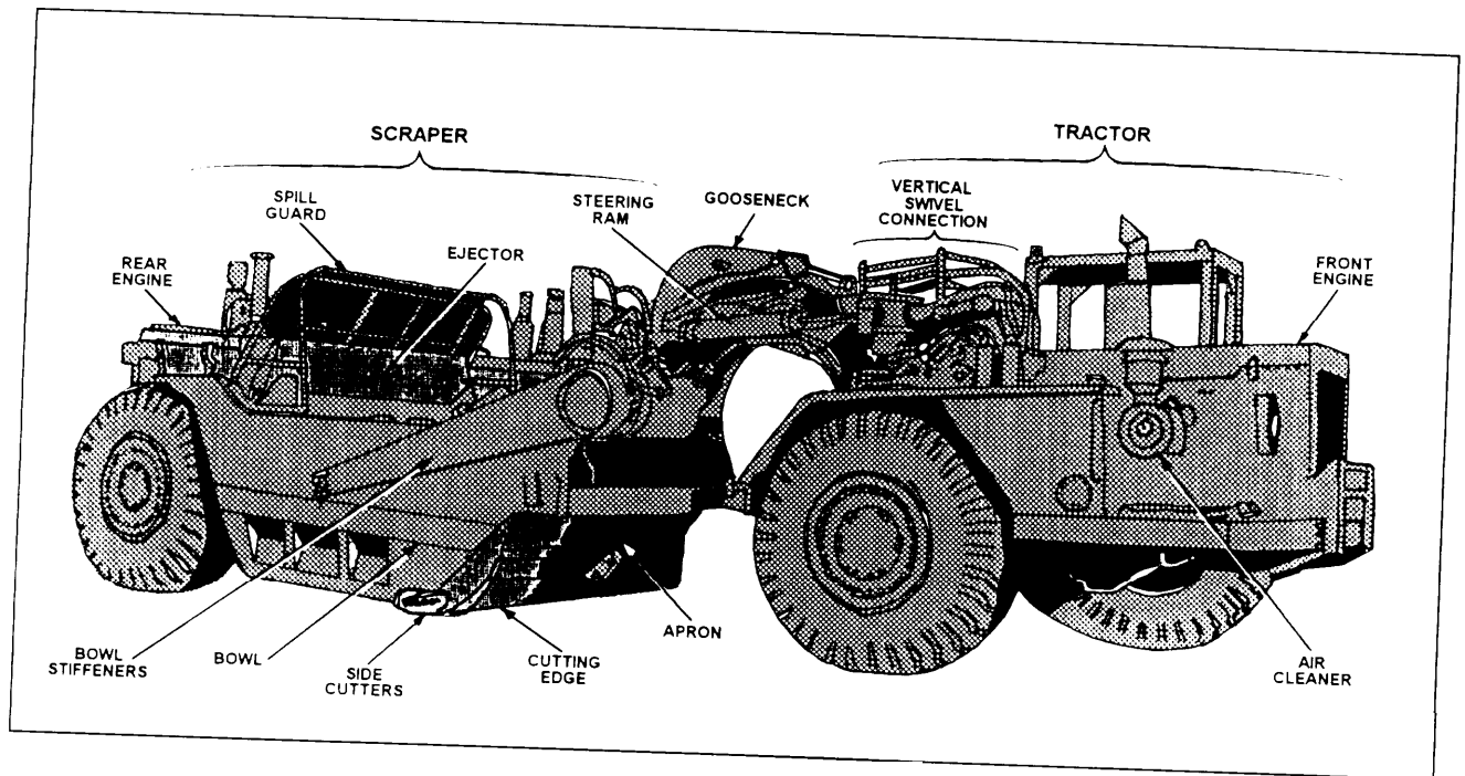
Figure 10-35.—Scrapper nomenclature.
