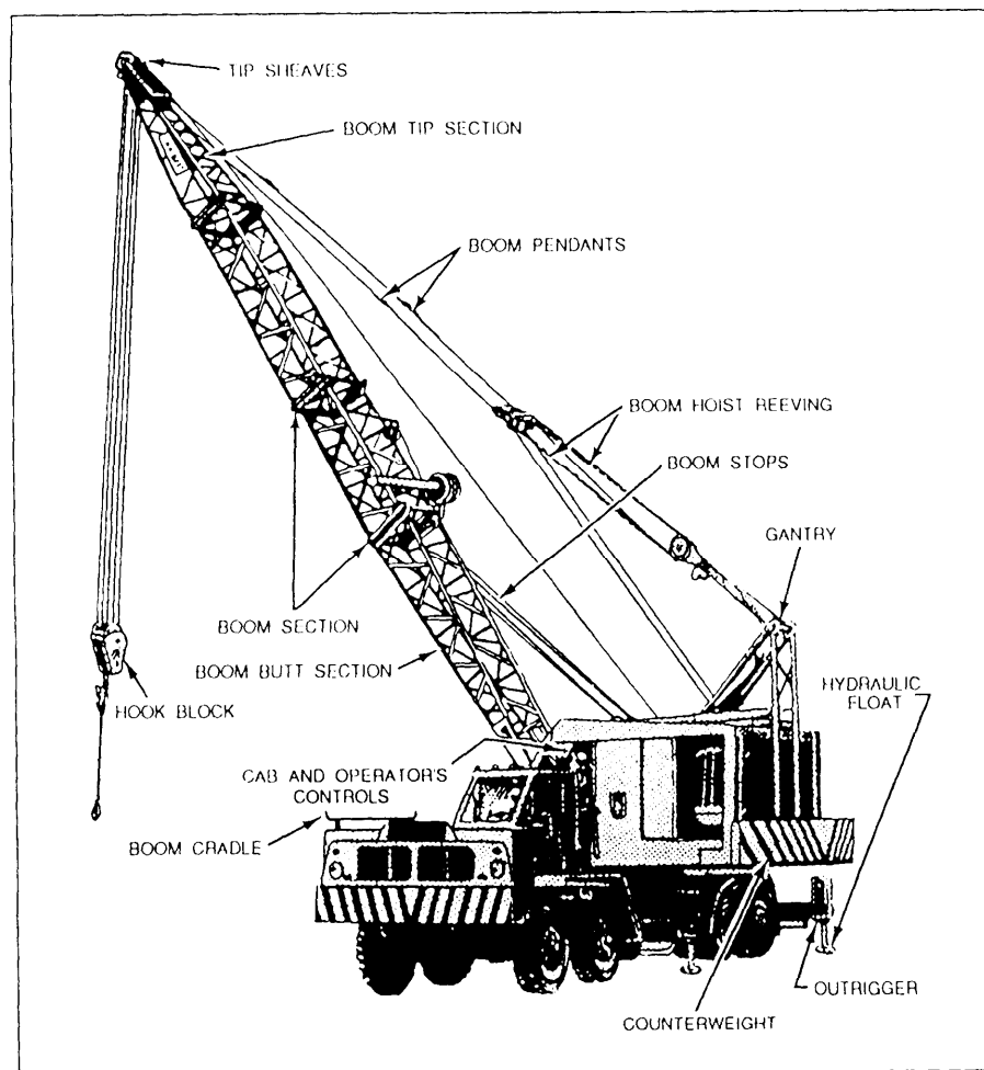
Figure 12-6.—Truck-mounted crane.
