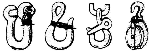
Figure 13-26.—Mousing.
