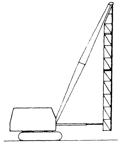
Figure 12-54.-Underhung leads.
