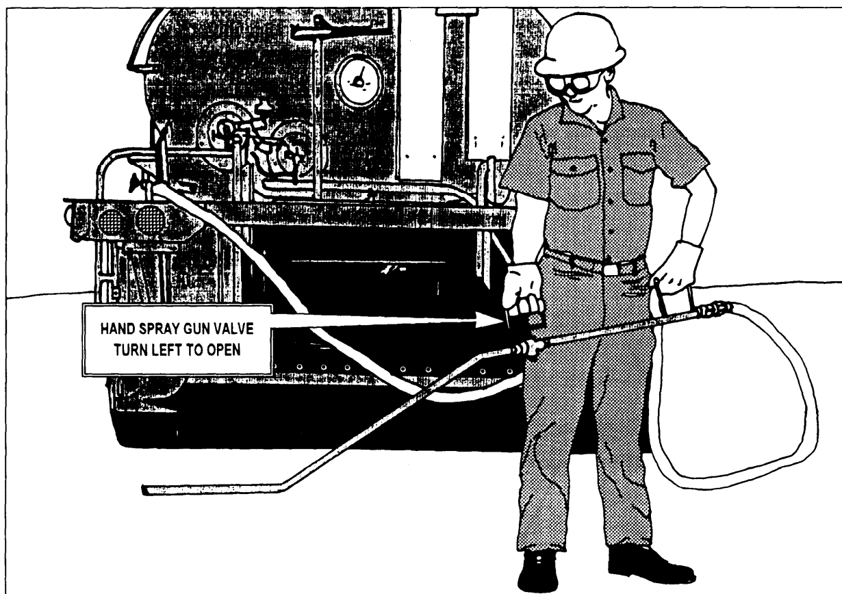
Figure 16-36.-Hand-spray application.
