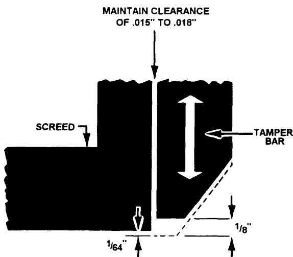
Figure 16-41. Tamping bar.
