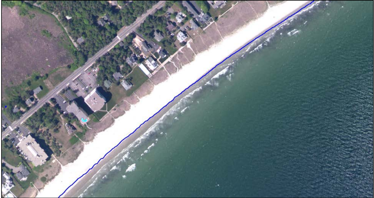
Figure 6-5. Lidar-derived mean high water shoreline (blue line) on top of aerial photo taken around the predicted time of mean high water
