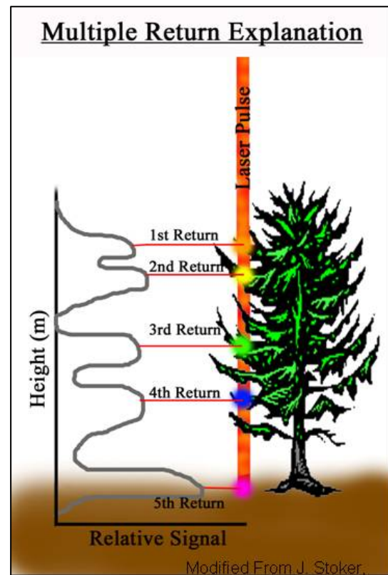
Figure 5-1. Multiple returns from single laser pulse
