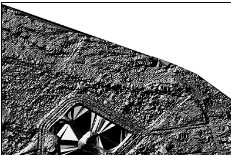
Figure 4-13. Hillshade
